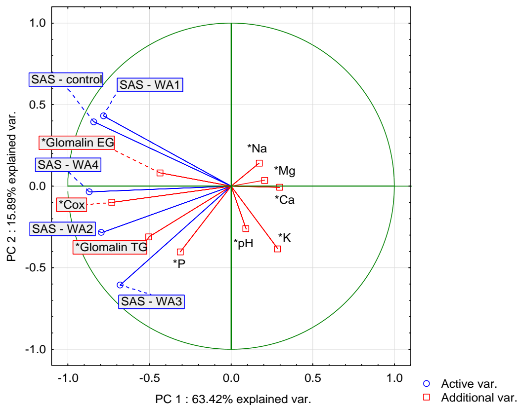
Figure 3 PCA biplot graph.
