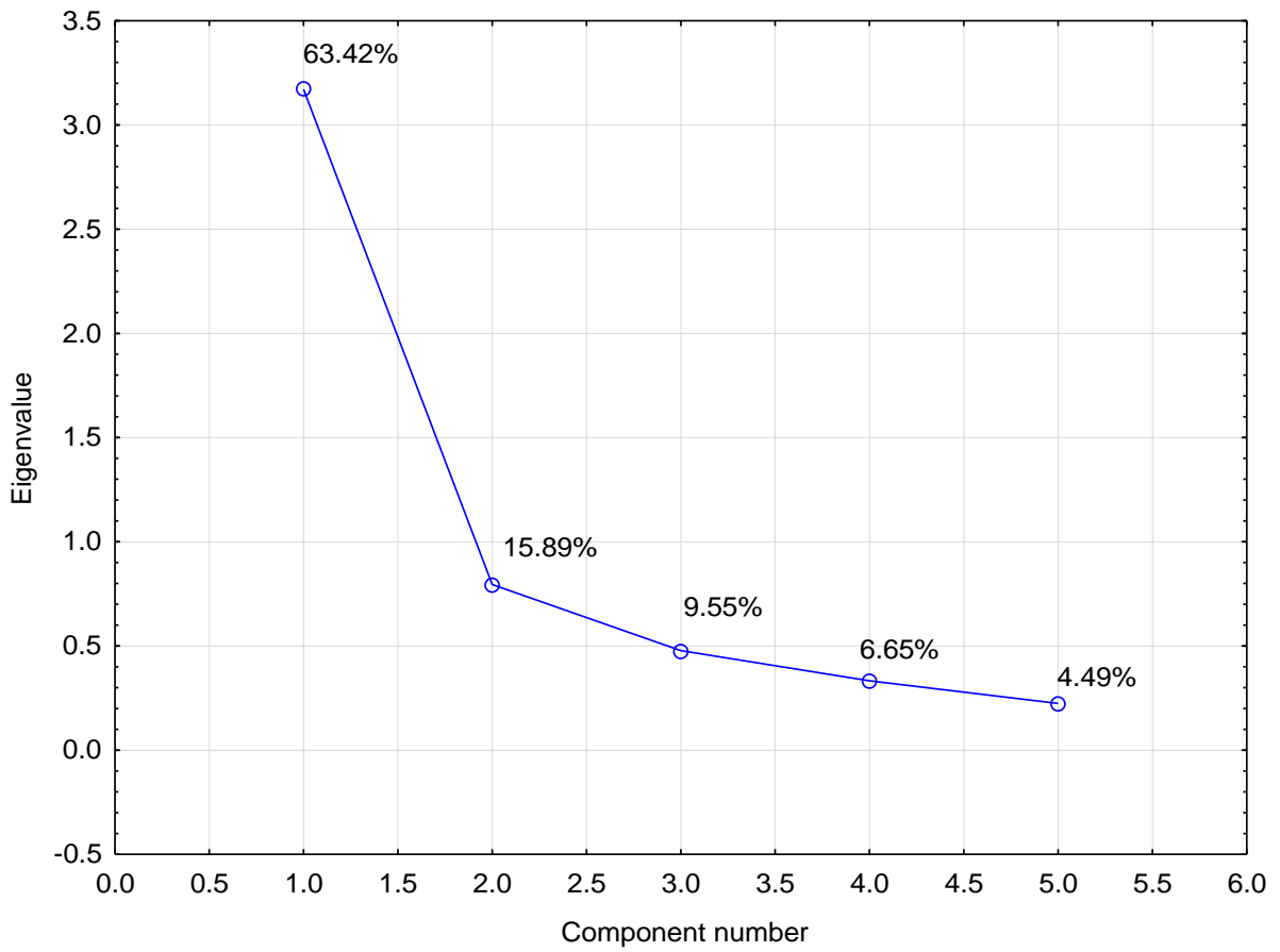
Figure F1e- PCA scree plot – graph of eigenvalues (variances) of all factors
