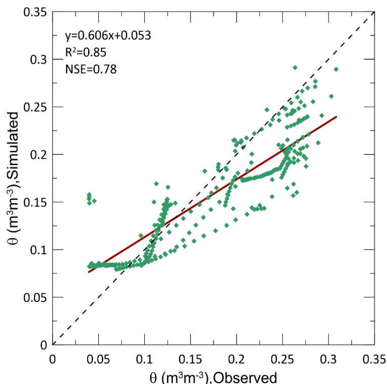
Figure 4: Relation between soil moisture content ( \theta ) values simulated and measured at SC4 location. The coefficient of determination ( R^2 ) and the Nash-Sutcliffe Efficiency (NSE) index are indicated.
