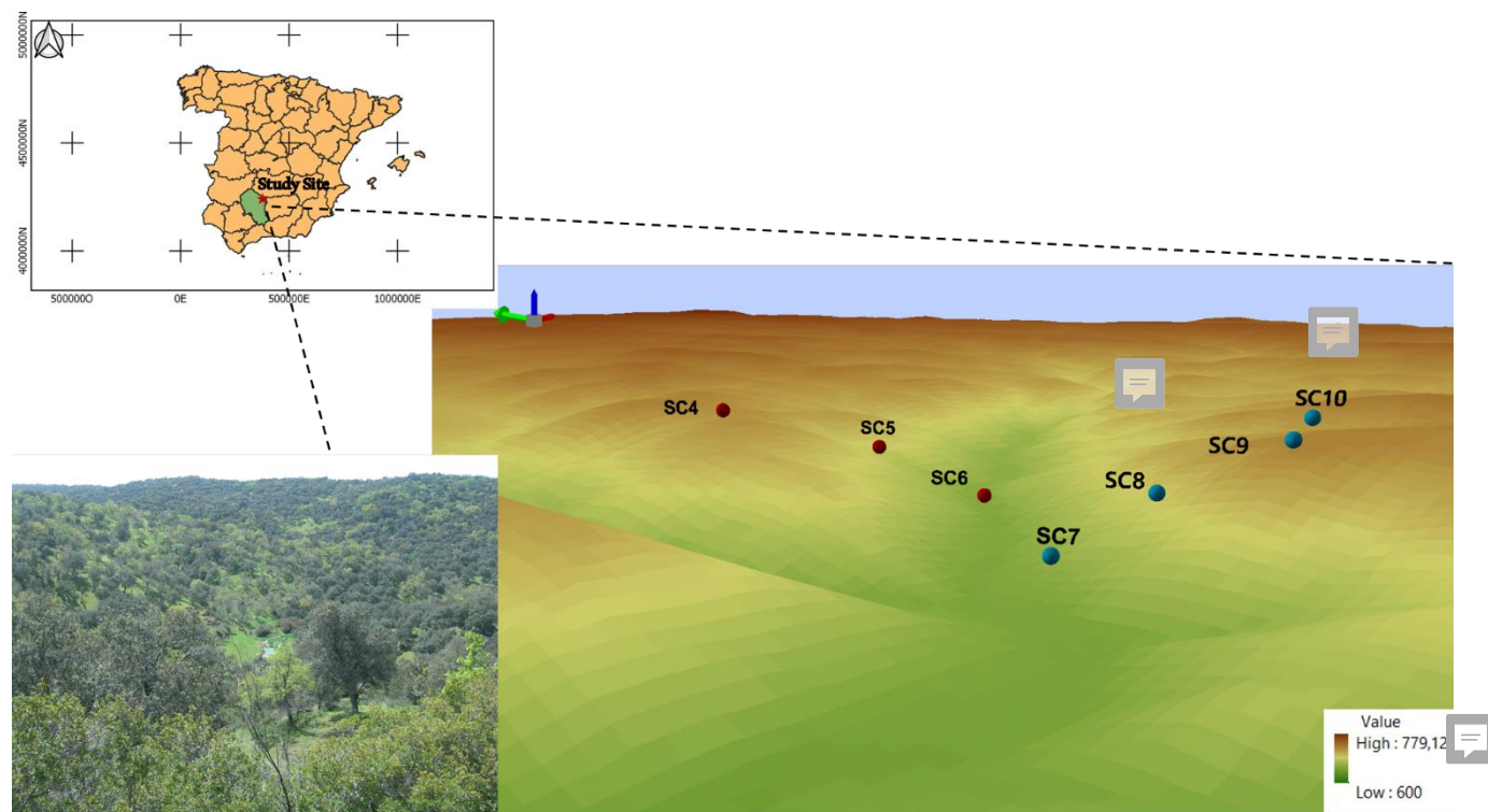
Figure 1: General location map of the study area and a detailed terrain map showing the location of the seven analyzed soil profiles along the catena with two opposing north-south facing slopes (respectively NFS and SFS, blue and red dots). The inset photo shows a landscape view of the study area. Note the green arrow indicates the north.
