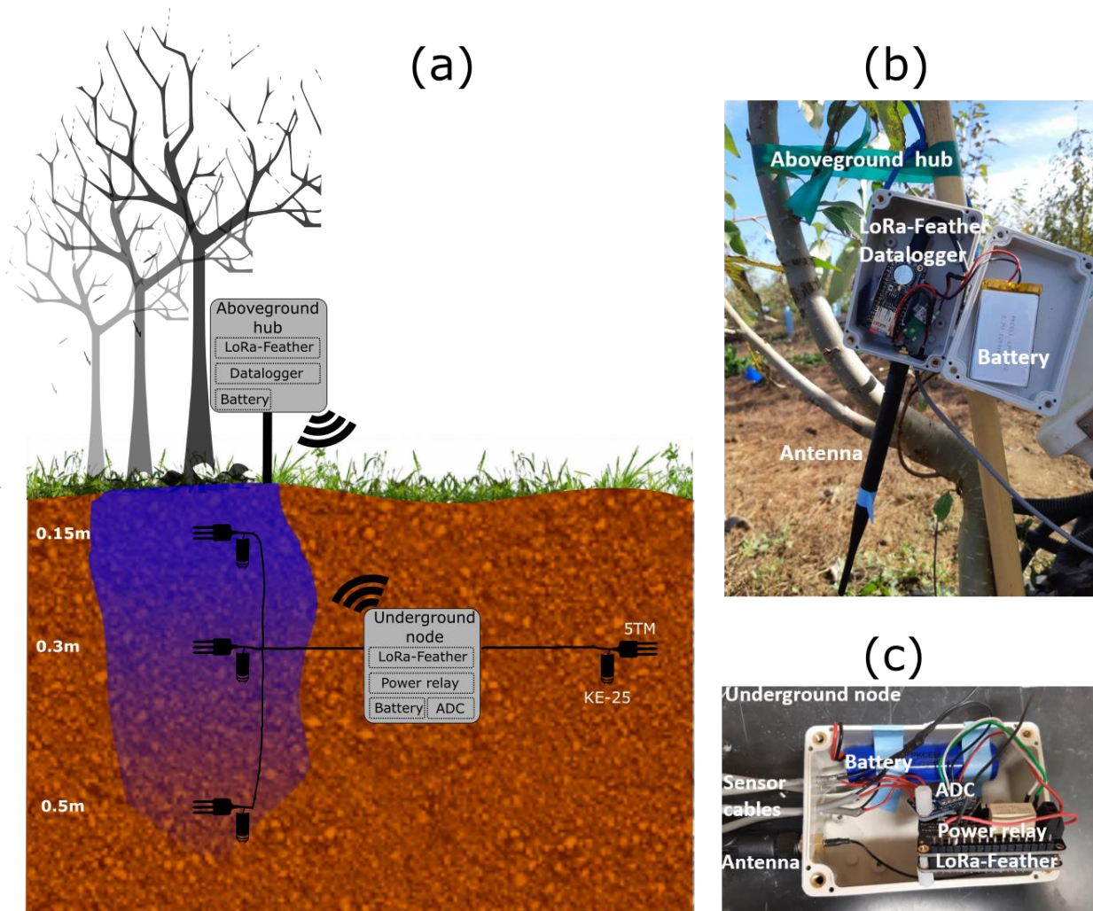
155 Figure 1: Scheme of the LoRa-WUSN experimental setup in the field (a), the components of the aboveground hub (b), and the underground node before coating (c).
