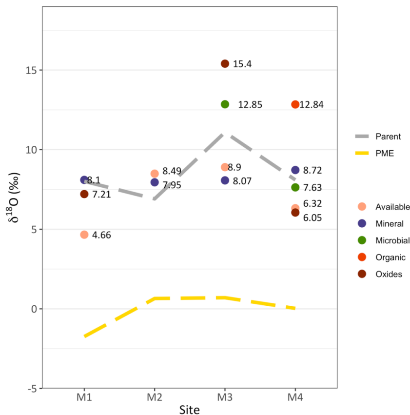
Figure 2: Isotopic values of oxygen in phosphate ( \delta^{18}\text{O}_P ) in different soil P pools along the Chamser Kangri glacier forefield chronosequence (<1, 25, 50 and > 100 years, for M1, M2, M3 and M4, respectively). The expected \delta^{18}\text{O} value of phosphate derived from Po hydrolysis due to phosphomonoesterases (PME, \delta^{18}\text{O}_{\text{PME}} , Eq. 2) is shown by the yellow discontinuous line, while the grey discontinuous line stays for the isotopic value of the parent material.
