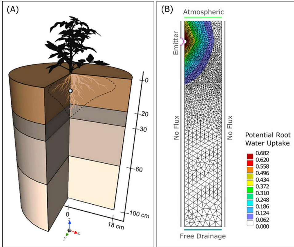
200 Figure 2 (A) 3D schematic representation of the domain geometry and material distribution. (B) Domain setup in Hydrus-2D showing the finite element mesh, related boundary conditions, and potential root water uptake rate distribution.
