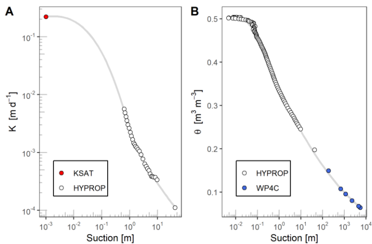
Figure 4 Plot of measured hydraulic conductivity (A) and water retention (B) for one of the topsoil ST-CC samples with the measurement instrument labeled. Grey lines are LOESS smooth trend lines.
