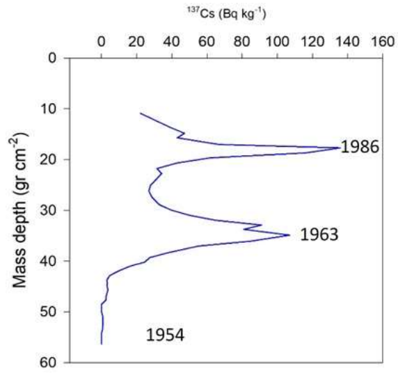
Supplementary Figure 1: Depth distribution of ^{137}\text{Cs} at the Zarivar lake sediment core showing two distinct peaks corresponding with 1963 and 1986.
