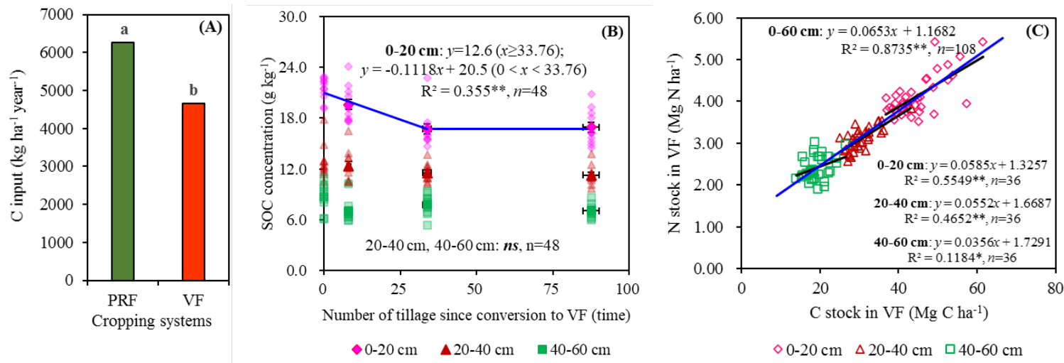
Figure 2: Organic C inputs in paddy rice-oilseed rape rotation and vegetable production(A), the relationship between SOC content and accumulative number of tillage operations since conversion to vegetable cropping system(B), and the relationship between soil N stock and soil C stock in the 0-20, 20-40, and 40-60 cm soil layers in the vegetable production(C). Error bars represent standard deviation. Significance levels *, P < 0.05 ; **, P < 0.01 ; ***, P < 0.001 ; ns, non-significant difference. VF, vegetable production; PRF, paddy rice-oilseed rape rotation.
