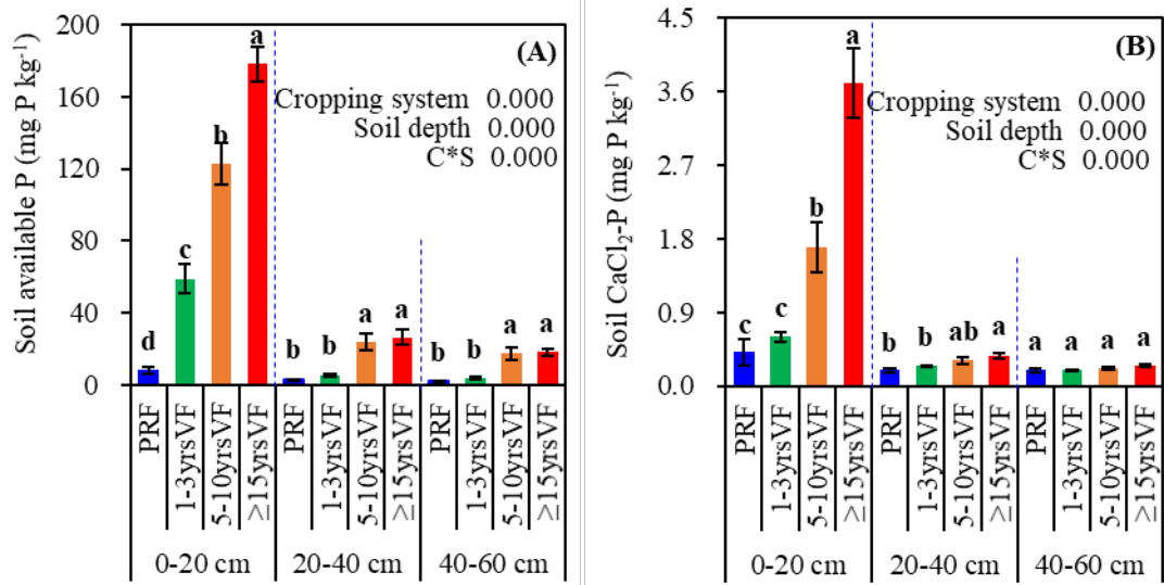
Figure 3: Changes in Soil available phosphorus (P) (A) and CaCl 2 -P (B) in the 0-20, 20-40, and 40-60 cm soil layers in the paddy rice–oilseed rape rotation and vegetable production converted from paddy-rape rotation in southwest China 1-3, 5-10, or ≥ 15 years ago. For each soil layer, different lowercase letters indicate significant differences at P < 0.05 . Error bars represent standard deviation. ANOVA results are shown at the top right corner. VF, vegetable production; PRF, paddy rice-oilseed rape rotation.
