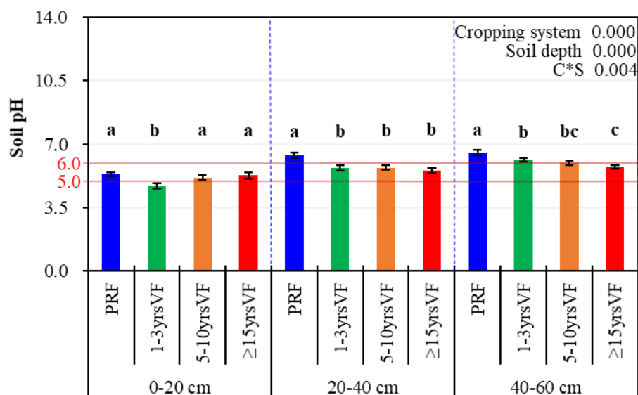
Figure 6: Soil pH in 0-20, 20-40, and 40-60 cm soil layers in the paddy rice-oilseed rape rotation and vegetable production converted from the paddy-rape rotation in southwest China 1-3, 5-10, or \geq 15 years ago. For each soil layer, different lowercase letters indicate significant differences at P < 0.05 among cropping systems. Error bars represent standard deviation. ANOVA result is shown at the top right corner. VF, vegetable production; PRF, paddy rice-oilseed rape rotation.
