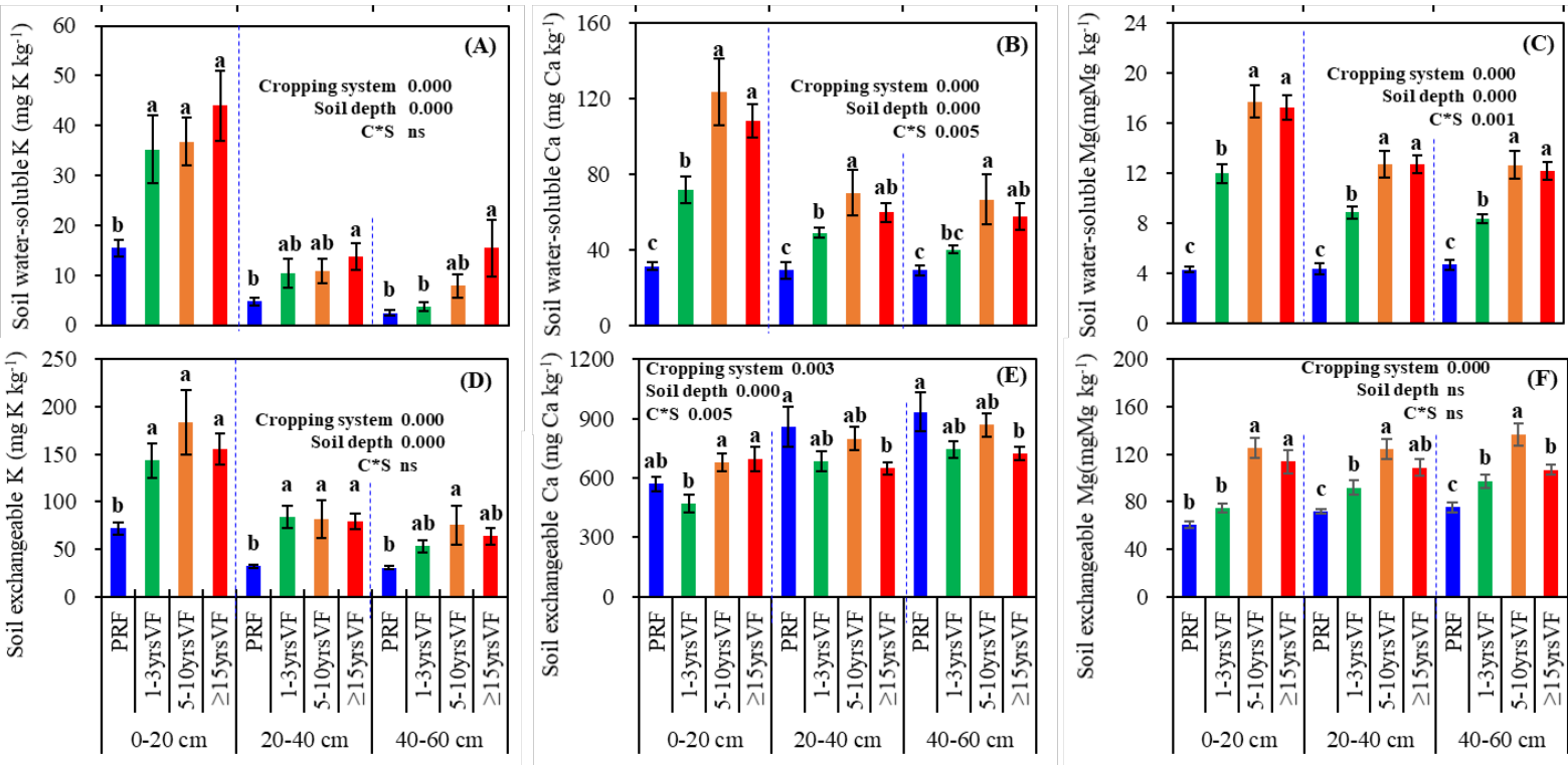
Figure 5: Soil water-soluble potassium(K) (A), water-soluble calcium(Ca) (B), water-soluble magnesium(Mg) (C), soil exchangeable (including the water-soluble fraction) K (D), exchangeable Ca (E), and exchangeable Mg (F) in 0-20, 20-40, and 40-60 cm soil layers in the paddy rice–oilseed rape rotation and vegetable production converted from paddy-rape rotation in southwest China 1-3, 5-10, or ≥ 15 years ago. For each soil layer, different lowercase letters indicate significant differences at P < 0.05 among cropping systems. Error bars represent standard deviation. ANOVA result is shown at the blank of plot: “ns” indicates no significant difference. VF, vegetable production; PRF, paddy rice–oilseed rape rotation.
