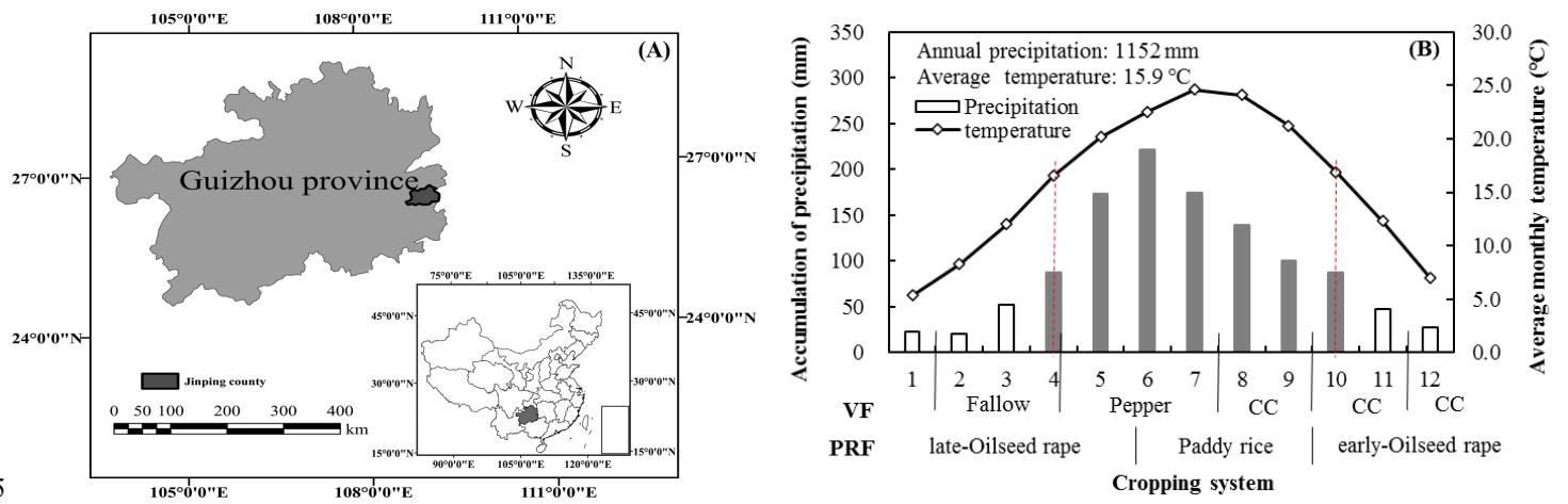
Figure 1: The Location (A), meteorological conditions (values averaged between 2007 and 2017), and typical cropping systems (B) of the study area. CC, non-heading Chinese cabbage; VF, vegetable production; PRF, paddy rice-oilseed rape rotation.
