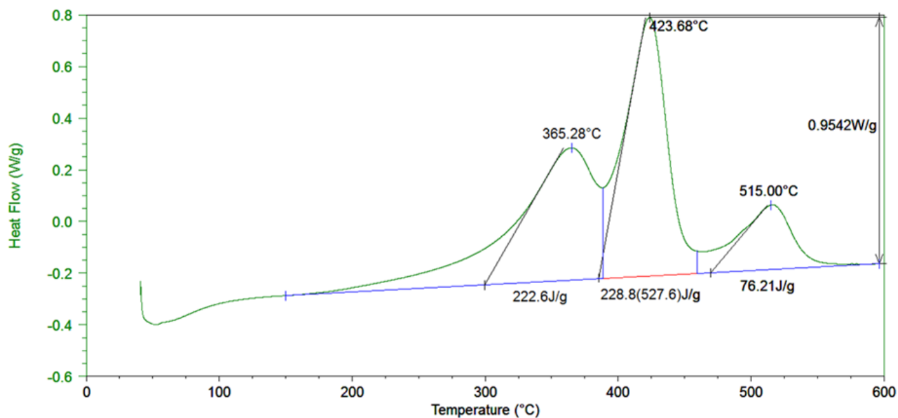
615 Figure 1. Measurement of characteristics from DSC thermograms (green line). After identification of peak maxima, peak height (W g -1 ) was measured as the maximum deviation from a linear baseline drawn between 150 and 600 °C, as illustrated for the main peak of the thermogram (0.9542 W g -1 ). Total heat release (527.6 J g -1 ) corresponds to the surface of the graph delimited by the linear baseline. Peak area (J g -1 ) was obtained by vertical drop between two adjacent peaks based on the position of the minima between two peaks. The black lines indicate the maximum rate of reaction associated to each maximum, and cross the baseline at the onset point (Temperature at which oxidation of the material starts).
