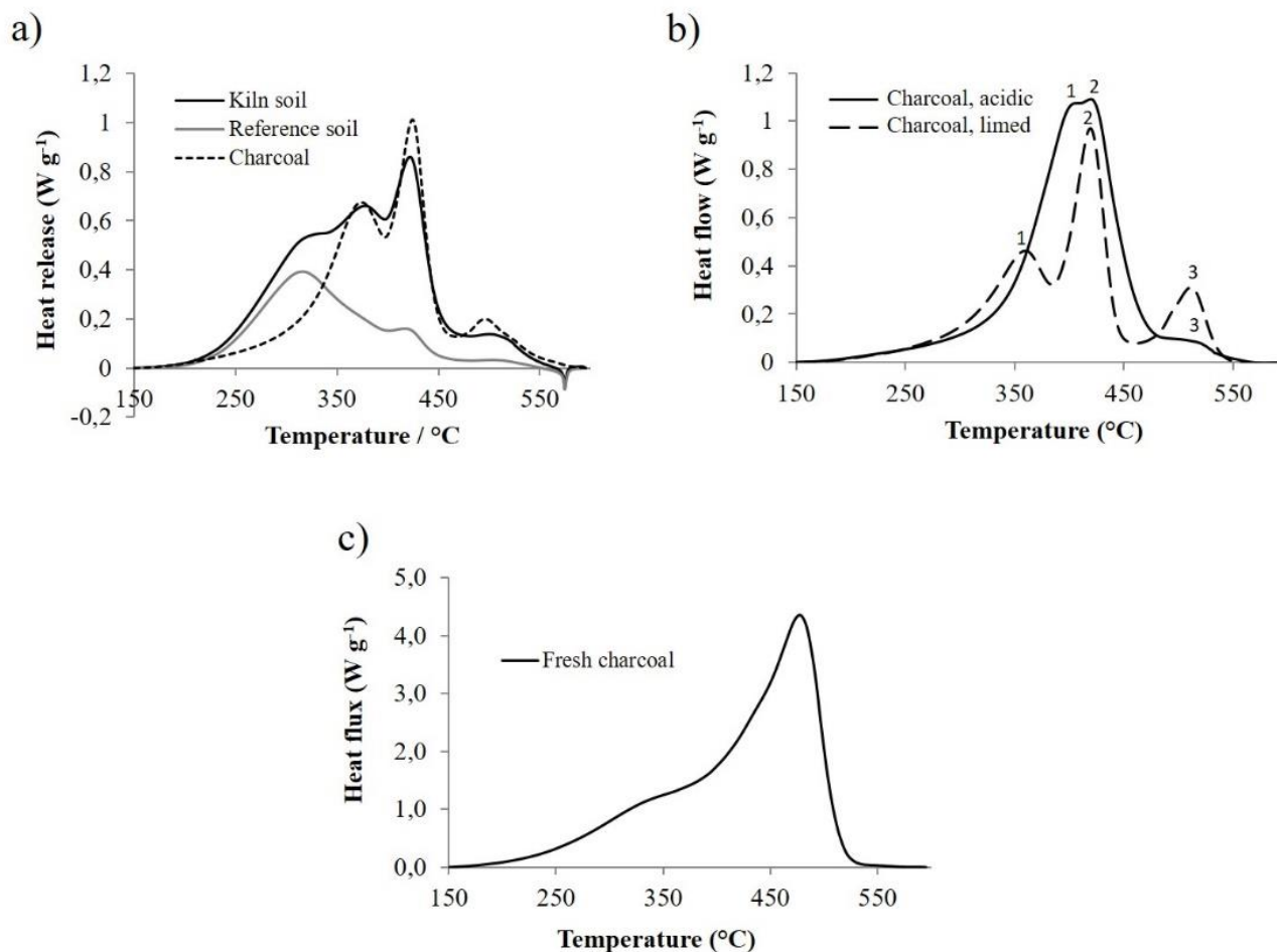
635 Figure 5. Differential scanning calorimetry thermograms of several charcoals; a) Thermogram of charcoal particles superimposed to the thermogram of the soil of the pre-industrial charcoal kiln site from which particles were extracted, and to the thermogram of adjacent reference soil (adapted from Hardy et al. , 2017a); b) Thermograms of charcoals extracted from an acidic forest soil and from a limed cropland soil. Numbers on the graph identify the maxima of exothermal peaks specific to the combustion of charcoal; c) Thermogram of a birch charcoal that was not aged in soil, produced in august 2012 in a traditional mound kiln.
