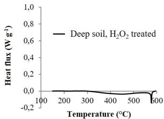
Figure 3. Differential scanning calorimetry thermograms of the subsoil (argic horizon) of a Haplic luvisol, H 2 O 2 treated.
