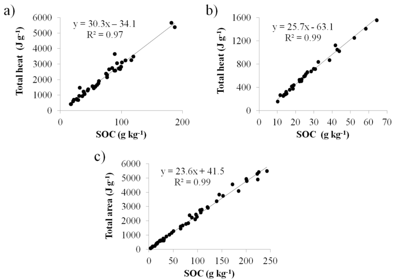
Figure 4. Total heat released between 150 and 600 °C from kiln and reference soils as a function of SOC content; a) forest soils of Wallonia; b) cropland soils of Wallonia; c) forest soils from Germany.
