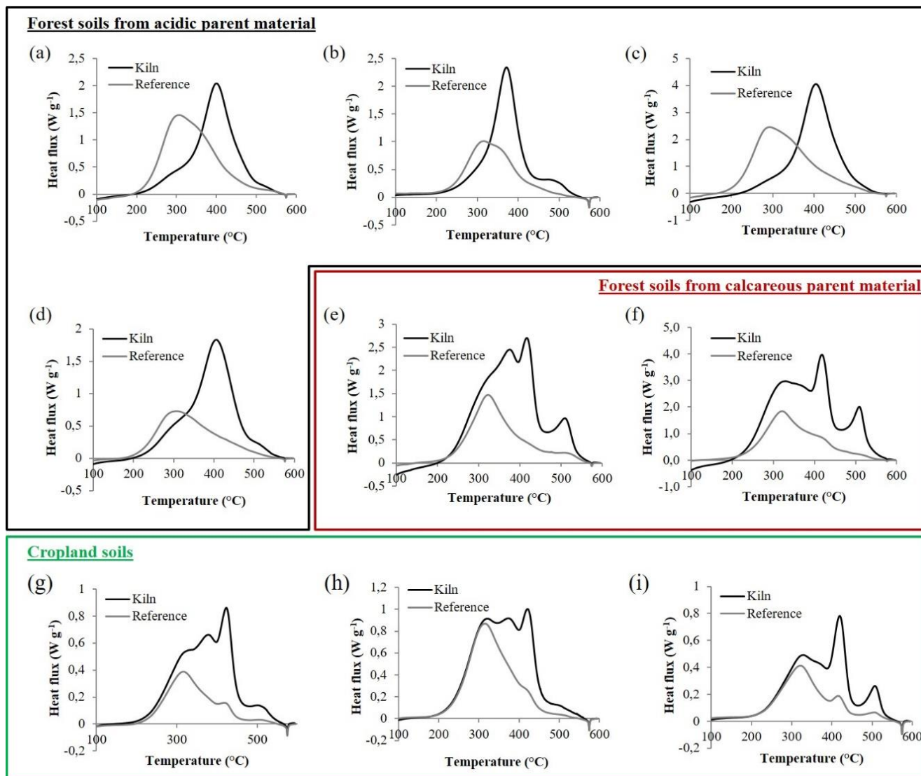
Figure 2. Differential scanning calorimetry thermograms of a representative selection of soils from pre-industrial charcoal kiln sites (black curves) and adjacent reference soils (grey curves). Four sites are located on (very) acidic forest soil (a, b, c, d), two sites located on calcareous forest soil (e, f) and three sites on cropland soils (g, h, i).
