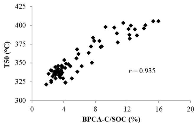
Figure 6. Temperature of 50 % heat release of bulk soils of Germany from the study of Borchard et al. (2014) against the fraction of C from BPCA (BPCA-C/SOC).
