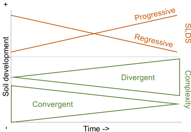
Figure 2: Illustration of evolutionary pathways related to soil-landscape development state (SLDS) and soil complexity.
