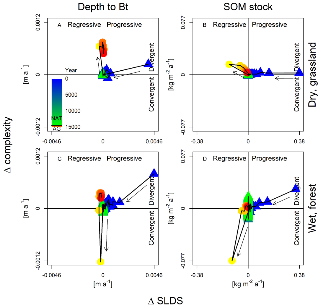
150 Figure 4: Changes in SLDS (X-axis) and complexity (Y-axis) for depth to Bt horizons (A, C) and SOM stocks (B, D) for both rainfall scenarios (dry: A, B; wet: C, D). The colors of the symbols indicate the year. The symbols themselves indicate the land use (triangles: natural, year 0-14500, blue to green colors; circles: agricultural, year 14500-15000, yellow to red colors). The timestep \Delta t over which the evolutionary pathways are calculated is 50 years for both land uses.
