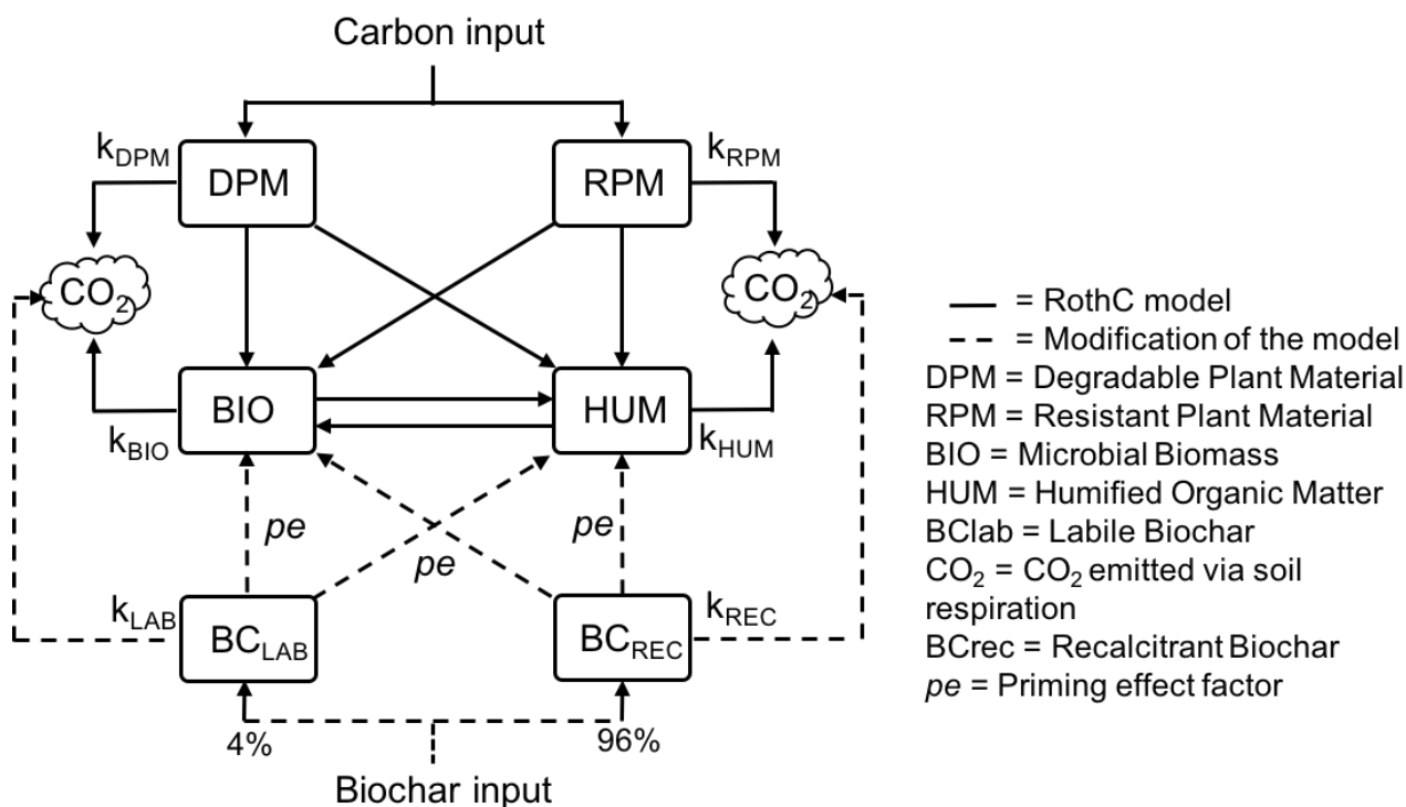
210 Figure 1. Modification of the RothC model with the inclusion of labile and recalcitrant biochar pools, and the priming effect on BIO and HUM. The CO 2 pool is assumed to be comparable to soil heterotrophic respiration.
