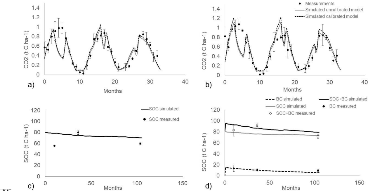
Figure 2. (a) Measured (circles) and simulated (lines) heterotrophic respiration, according to the control model before calibration (solid lines) and after calibration (dashed lines), across a three year period (2012-2014). (b) Measured (circles) and simulated heterotrophic respiration, according to the biochar model, before calibration (solid lines) and after calibration (dashed lines), across a three year period (2012-2014). (c) Calibration (dashed line) and validation (solid line) of control model against SOC measurements (circles) taken in 2013, 2015, 2020. (d) Measured (unfilled circles), simulated SOC (grey solid line) and SOC with biochar-C (black solid line) in model validation. Biochar-C (filled circle) and simulated biochar-C (dashed line) represent the amount of biochar in soil without native SOC. Month of simulation 0 corresponds to March 2012, month of simulation 105 corresponds to December 2020.
