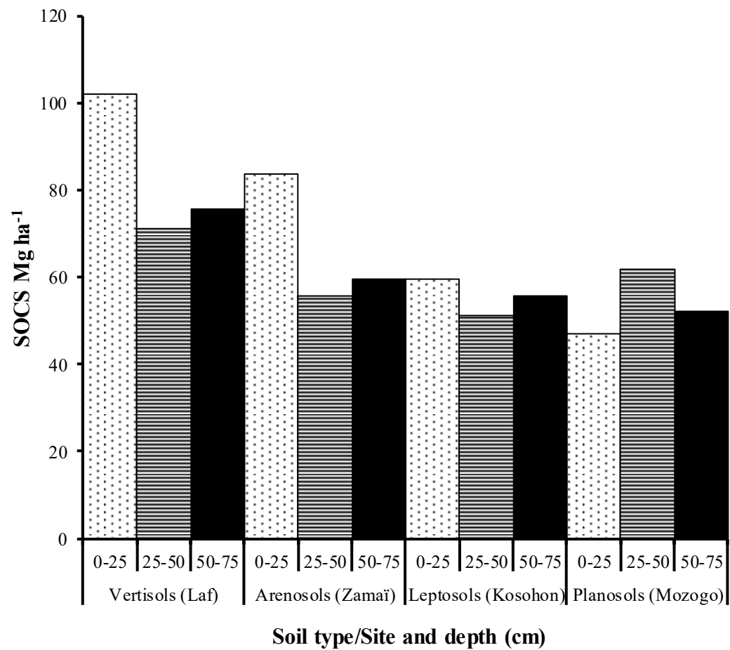
720 Fig. 3. Variation of SOCS along the soil profiles in the study sites.
