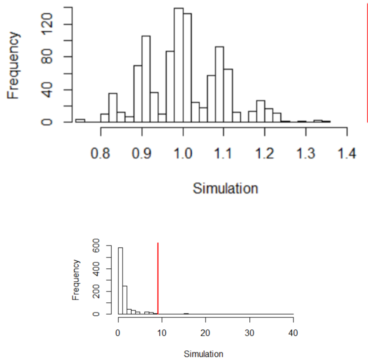
Figure 1: RMS's simulation ratios in relation to the observed ratio (red) at 5-10 cm depth
