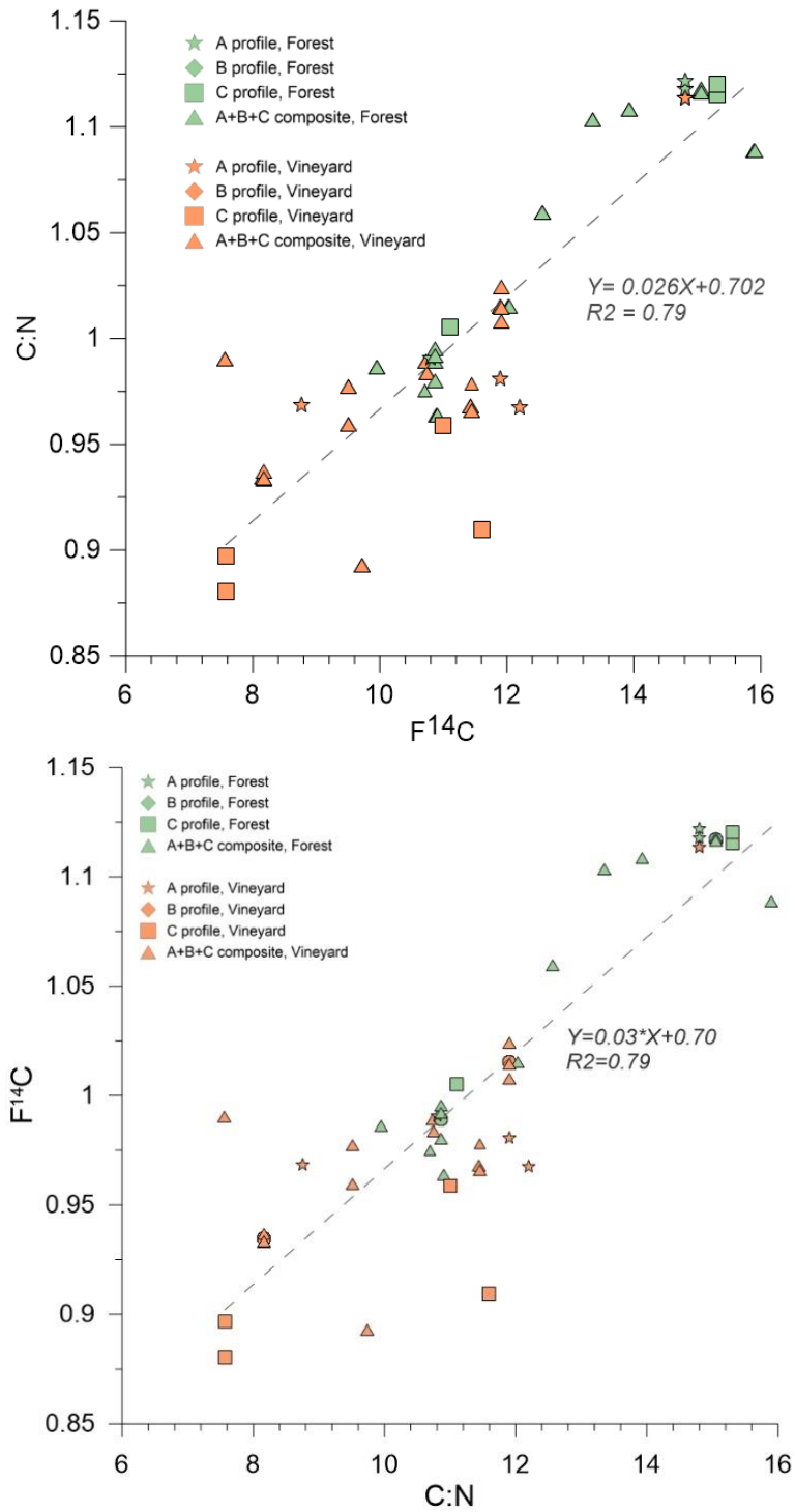
Figure 4: Correlation between the F14C and C:N ratio. The correlation was calculated on composite samples (F14C) and the average for the 3 profiles A, B and C (C:N), as well as on simple samples of profiles A, B and C, from the forest (green) and vineyard (orange) soils
