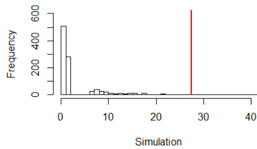
Figure 2: RMS's simulation ratios in relation to the observed ratio (red) at 40-50 cm depth
