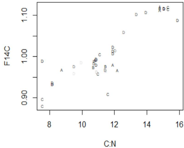
Figure 5: F14C as a function of C:N. The letters correspond to the faces of the pit, their colour to their depth (the lighter the colour, the deeper the sample).
