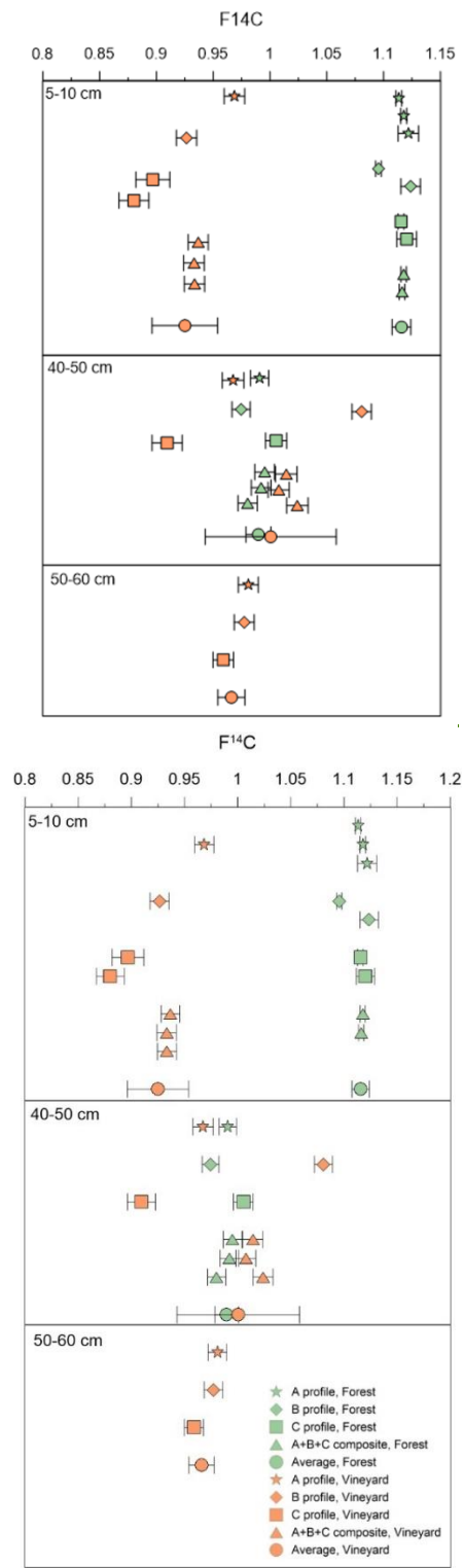
Figure 3 : Comparison of intra-layer F^{14}C heterogeneity at three depths (5-10, 40-50 and 50-60 cm) in forest and vineyard soils. F^{14}C data were obtained for profiles A (star), B (diamond), C (square), composites A+B+C (triangle) and the average of these data (round), in forest (green) and vineyard (orange) soils. Error bars represent the analytical error for the profiles A, B and C and the standard deviation effor the mean .
