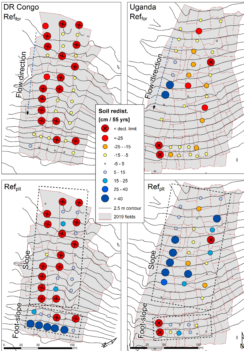
Figure 5: Soil redistribution derived from ^{239+240}\text{Pu} measurements using a mass balance model. Two different reference inventories (upper: \text{Ref}_{\text{for}} = mean forest reference; lower: \text{Ref}_{\text{plt}} mean cropland plateau reference) in two cropland areas of the White Nile-Congo rift region (left: DR Congo, right: Uganda) were used for calculation.
