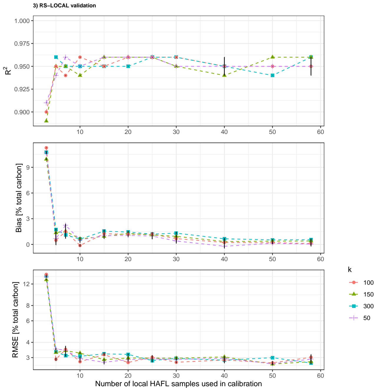
Figure D1. R^2 , bias and RMSE (% total carbon) of the validation of RS-LOCAL modelling approaches using different numbers of local HAFL samples in model calibration, when altering the RS-LOCAL parameter k . RMSE is on a logarithmic scale.
