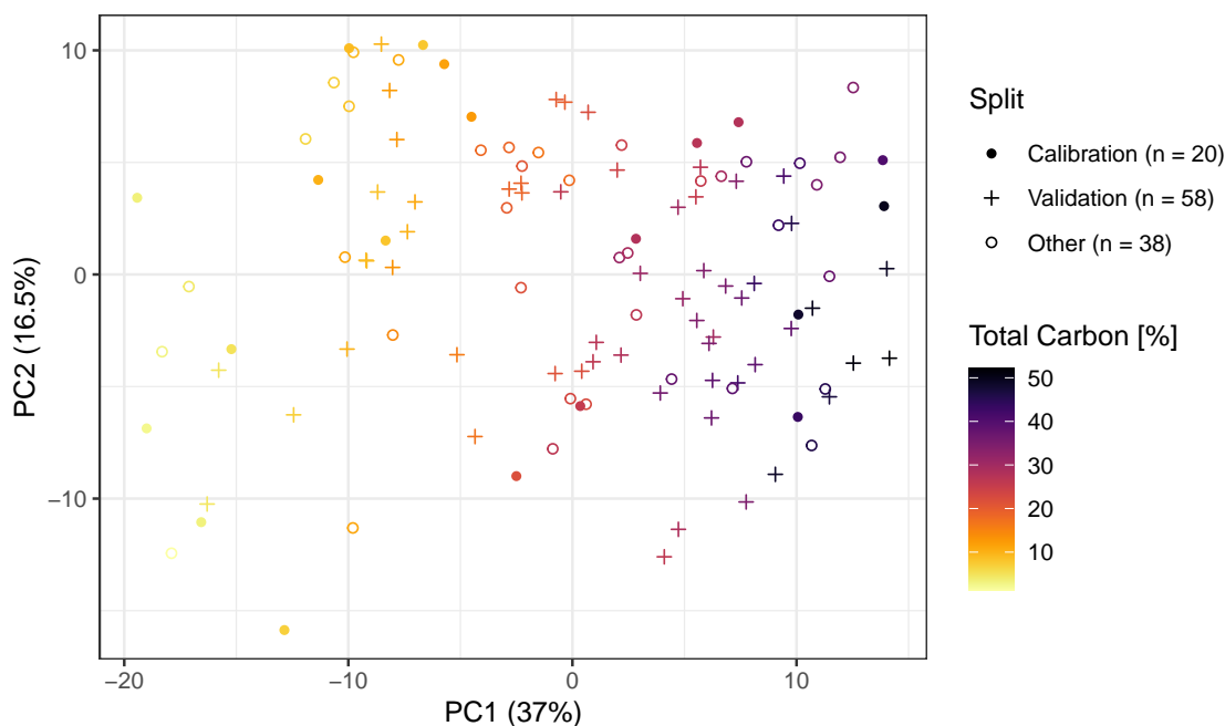
Figure 4. PC1 vs. PC2, computed via scaled and centered PCA, of the pre-processed local HAFL soil spectra ( n = 116 ) colored by total carbon content [%]. The axis labels show the relative amount of variance explained [%] in parentheses. In this example, n = 20 representative samples were selected using the KS algorithm for calibrating a local model.
