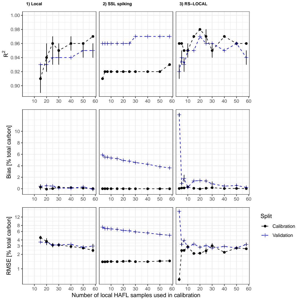
Figure 7. R 2 , bias and RMSE values in % total carbon (RMSE in logarithmic scale) vs. the number of local HAFL samples used in local HAFL (1), local combined with SSL (2) and RS-LOCAL subsets, where k = 100 (3). Error bars represent the SD between resampled repeats and where not present, there was no variation in the respective summary statistic across five repeats. Dashed lines between data points do not represent real measurements and are only for visual guidance.
