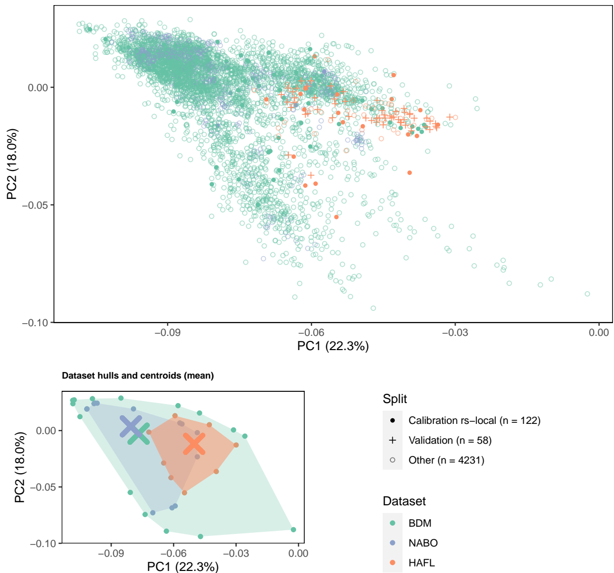
Figure 5. PC1 vs. PC2 and the convex hulls and centroids (mean) in PCA space of the pre-processed soil spectra of the local HAFL dataset ( n = 116 ) and the BDM and NABO datasets, which make up the current Swiss SSL ( n = 4295 ). Here, the PCs were computed via unscaled and uncentered PCA since it better showed the data distribution than a scaled and centered PCA. The axis labels show the relative amount of variance explained [%] in parentheses. In this example, the same representative local HAFL samples ( n = 20 ) selected in Figure 4 were used by RS-LOCAL to subset representative samples from the SSL ( n = 102 ), which were used together for model calibration ( n = 122 ).
