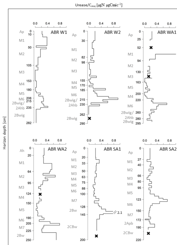
Figure 10: Depth profiles of Urease/ C_{mic} ratio of selected colluvial profiles. “x” = not analysed.
