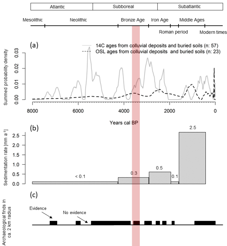
640 Figure 15: Summed probability density (SPD) curves from AMS- ^{14}\text{C} and OSL ages (a); sedimentation rate by depositional ages (OSL) and related to archaeological periods (b); Evidence of archaeological finds within a radius of 2 km from the Anselfingen settlement site (c). Red bar marks the Middle Bronze Age period.
