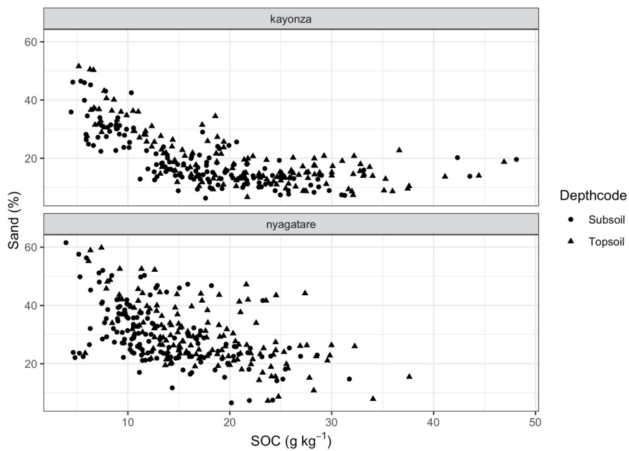
225 Figure 5: Relationship between sand content and soil organic carbon (SOC) for both top and sub soil samples at Kayonza and Nyagatare LDSF sites.
