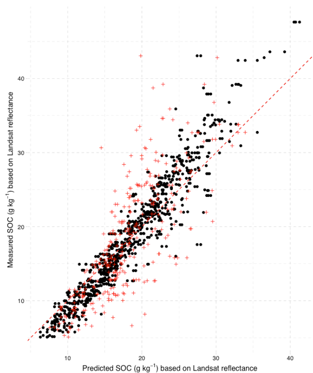
275 Figure 9. Predicted vs measured SOC based on predictions made from Landsat 8 reflectance for the two study sites. The black dots are training data, while the red crosses show independent validation results.
