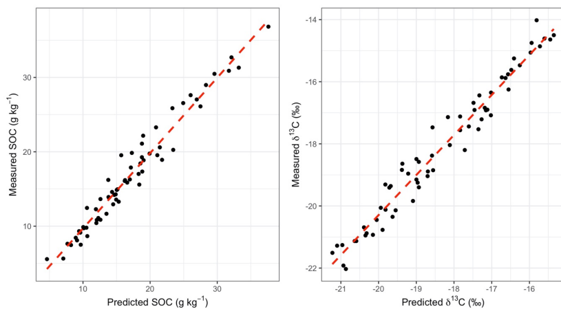
210 Figure 3. Predicted vs measured SOC and d13C based on MIR spectra for the two sites included in the study.
