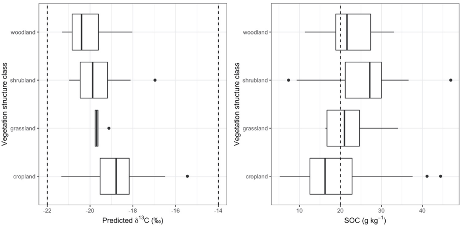
Figure 6: Boxplots of \delta^{13}\text{C} values and SOC content in topsoil for each vegetation structure class. Dotted vertical lines at -22 and -14 ‰ indicate the C3 and C4 dominated systems, respectively. The dotted line at 20 g kg -1 SOC is to indicate a threshold for agricultural productivity in humid areas.
