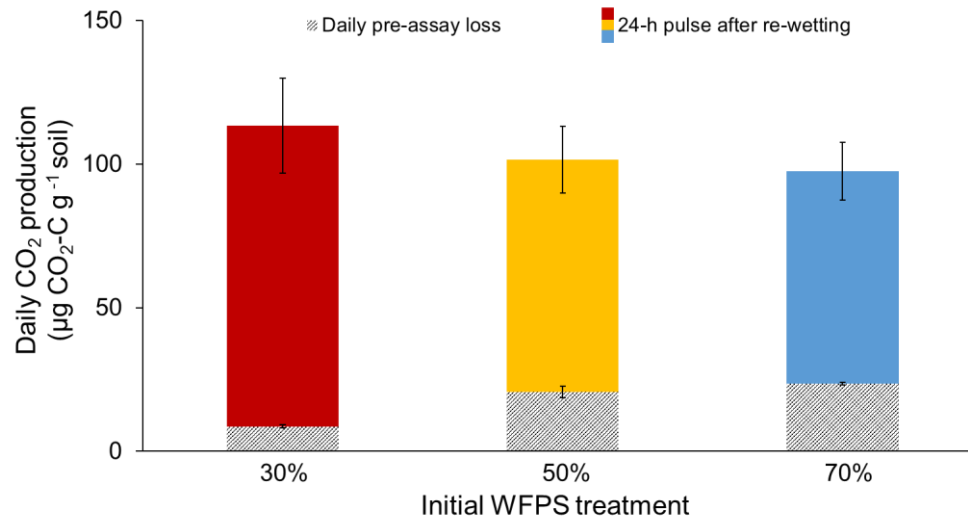
140 Fig 3. Daily CO 2 production rates for each initial water-filled pore space (WFPS) treatment. Lined bars represent the average daily rate of pre-assay CO 2 loss during a 3-day dry-down period and solid bars represent the 24-h CO 2 pulses after re-wetting the air-dried soil. Together both bars represent the 24-h CO 2 pulse corrected for pre-assay losses of CO 2 during dry-down. Error bars represent standard deviation, which was calculated based on bootstrap error propagation for the daily pre-assay losses.
