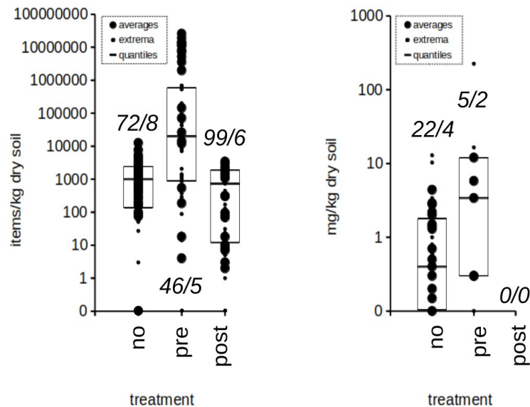
Figure 4: Quantities of MP measured after density fractionation without treatment of SOM (no), with pre-treatment (pre) and post-treatment (post). Big dots mark median and mean concentrations measured in worldwide field experiments, small dots the related extreme values or standard deviations, strong horizontal lines the overall medians and narrow lines the 25 % and 75 % quantile. Italic numbers indicate the underlying number of sampling sites / studies.
