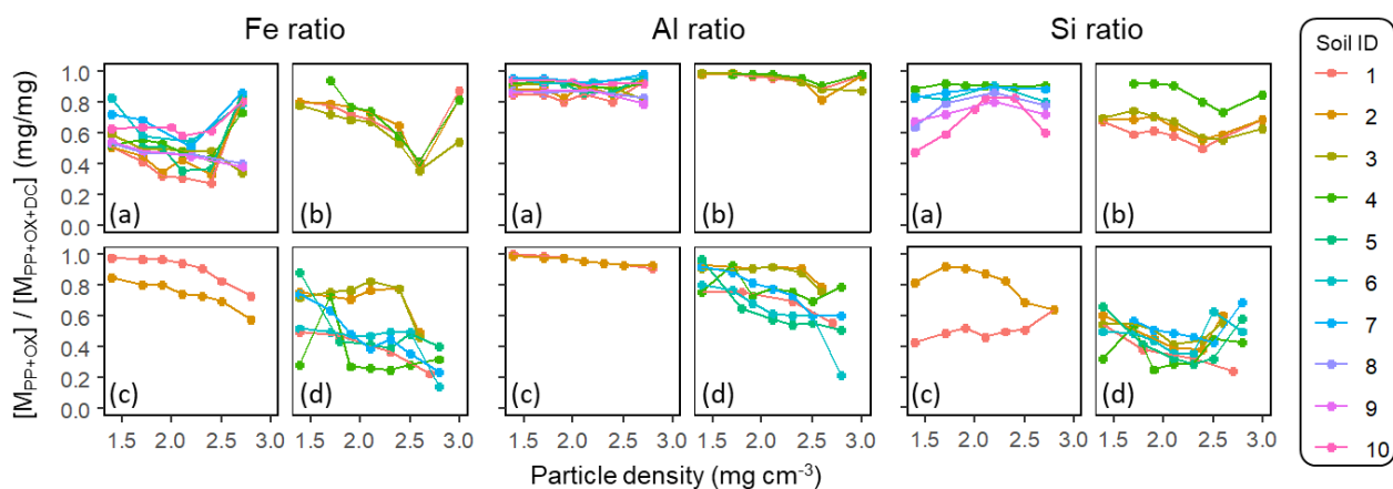
980 Figure A4: Proportion of total extractable Fe (left), Al (center), and Si (right panels) present as pyrophosphate- plus oxalate-extractable phases. This ratio obtained from each density fraction was shown along the density gradient for allophanic Andisols (a), non-allophanic Andisols (b), Spodosols (c), and crystalline mineralogy group (d). Each symbol represents individual soil sample ID in Table 1.
