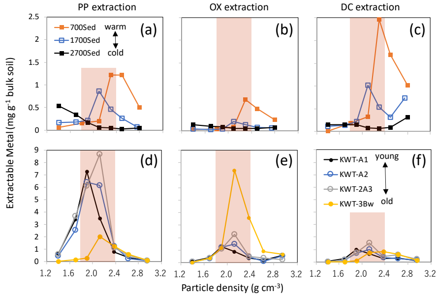
1025 Figure A8: The distribution of the extractable metal phases (Al+0.5Fe) along the particle density gradient for two soil series. Upper three plots show PP- (a), OX- (b), and DC-extractable metals (c) for three A horizon soils under tropical forest along an elevation gradient from a weathered soil under warm climate at 700 m (sample ID: C5), moderately weathered soil at 1700 m (C6), and much less weathered soil at 2700 m (C7). The lower panels (d, e, f) showed surface and buried horizons of a non-allophanic Andisol profile (sample ID: N1-N4) that received multiple tephra deposits. Shaded zones show the meso-density range.
