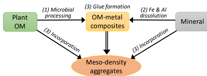
945 Figure 9: Conceptual illustration of meso-density aggregate formation. Three main processes are (1) microbial processing of plant-derived organic matter, (2) metal dissolution via chemical weathering, and (3) the formation of organo-metallic glue which promote meso-density microaggregate formation by incorporating some of POM and mineral.
