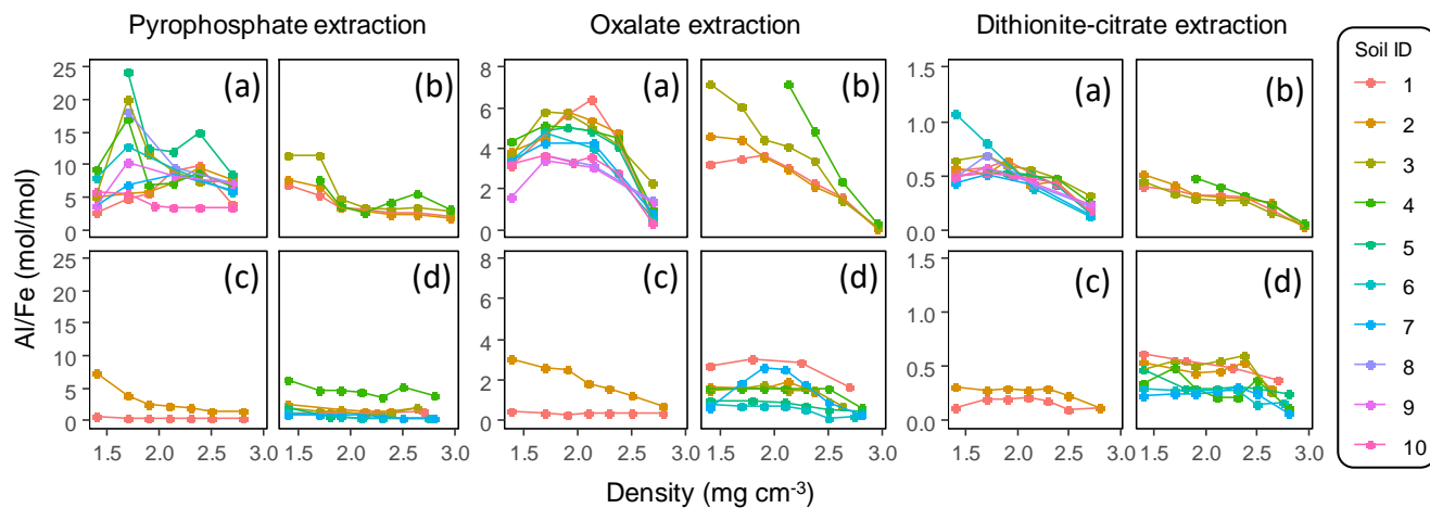
990 Figure A5: Molar Al-to-Fe ratio of each extractable phase from each density fraction along the density gradient. The ratio was shown for initial pyrophosphate (left four plots), subsequent acid oxalate (middle four plots), and final dithionite-citrate extractions (right four plots) were shown for Allophanic Andisols (a), non-allophanic Andisols (b), Spodosols (c), and crystalline mineralogy group (d). Each symbol represents individual soil sample ID in Table 1.
