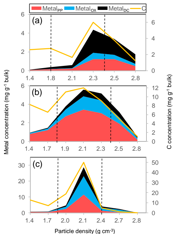
940 Figure 8: The distribution of the extractable metal phases (Al+0.5Fe) on left Y axis and that of C on the right Y axis along the density gradient for three undisturbed forest soils. A kaolinitic Ultisol (O-5 in Table 1) developed from sedimentary rock under tropical wet climate (a), a Spodosol Bhs horizon (S-2) with quartz and plagioclase rich mineralogy from glacial till under cool temperate moist climate (b), and an allophanic Andisol (A-10) from tephra under warm temperate moist climate (c). Vertical dotted lines show the meso-density range.
