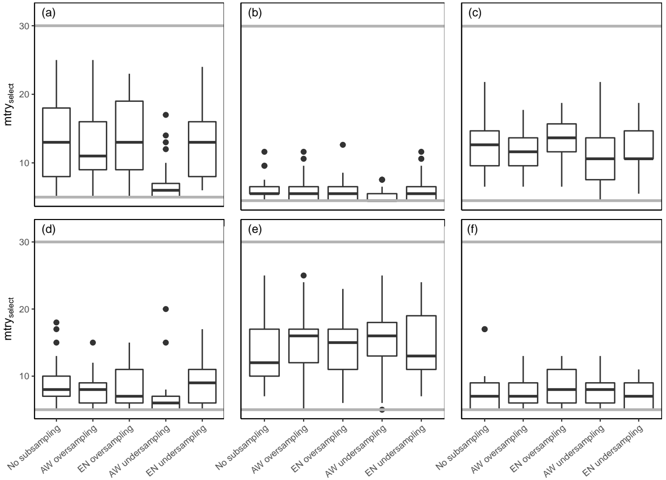
Figure 9. Results of the model tuning procedure to find the best performing mtry values ( mtry_{select} ) under different subsampling approaches. (a), (b) and (c) show the results of the clay, silt and sand models at 10 cm depth, while (d), (e) and (f) show the same texture classes at 70 cm depth. Grey lines correspond to the tested mtry parameter range
