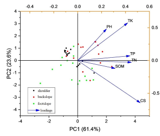
Figure 4: Eigenvectors from the principal component analysis (PCA) of the first two components.
