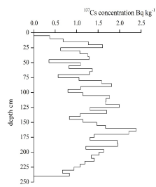
Figure 3: 137 Cs depth distribution features in depression bottom.
