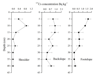
Figure 2 : 137 Cs concentration distribution features at different hillslope positions.
