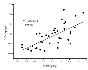
Figure 5: Linear correlation between 137 Cs and SOM (Soil Organic Matter) content.
