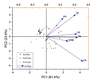
Figure 4: Eigenvectors from the principal component analysis (PCA) of the first two components.
