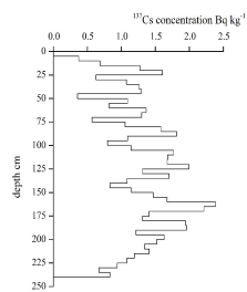
Figure 3: ^{137}\text{Cs} depth distribution features in depression bottom.
