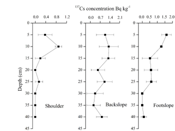
Figure 2 : ^{137}\text{Cs} concentration distribution features at different hillslope positions.
