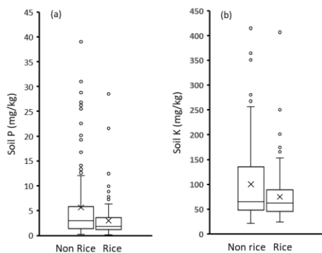
Fig 5. (a) Available P and (b) Extractable K concentrations across seven watersheds.
