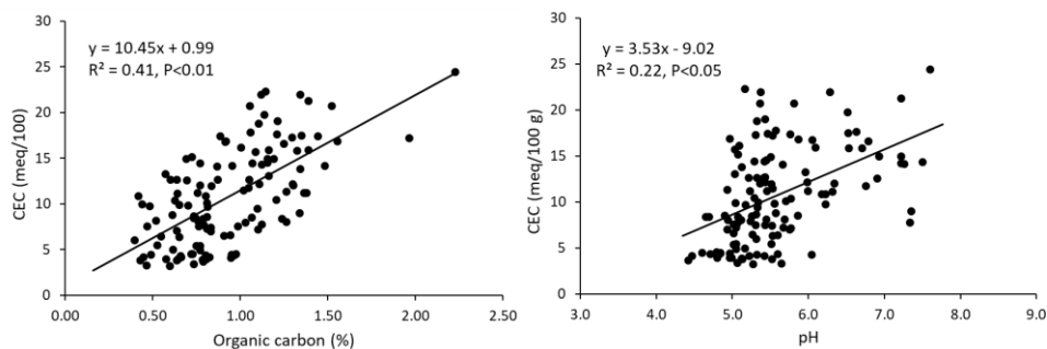
Fig 4. The relationship between cation exchange capacity and organic carbon and pH in soils across seven EIP watersheds.
