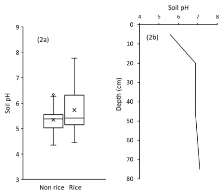
Fig. 2. Soil pH w in (a) surface soil across 7 EIP watersheds and (b) the mean of 54 rice field soil profiles at Purulia District.
