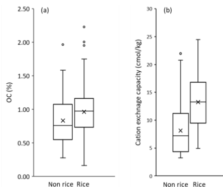
170 Fig 3. (a) Soil organic carbon and (b) cation exchange capacity across seven EIP watersheds.
