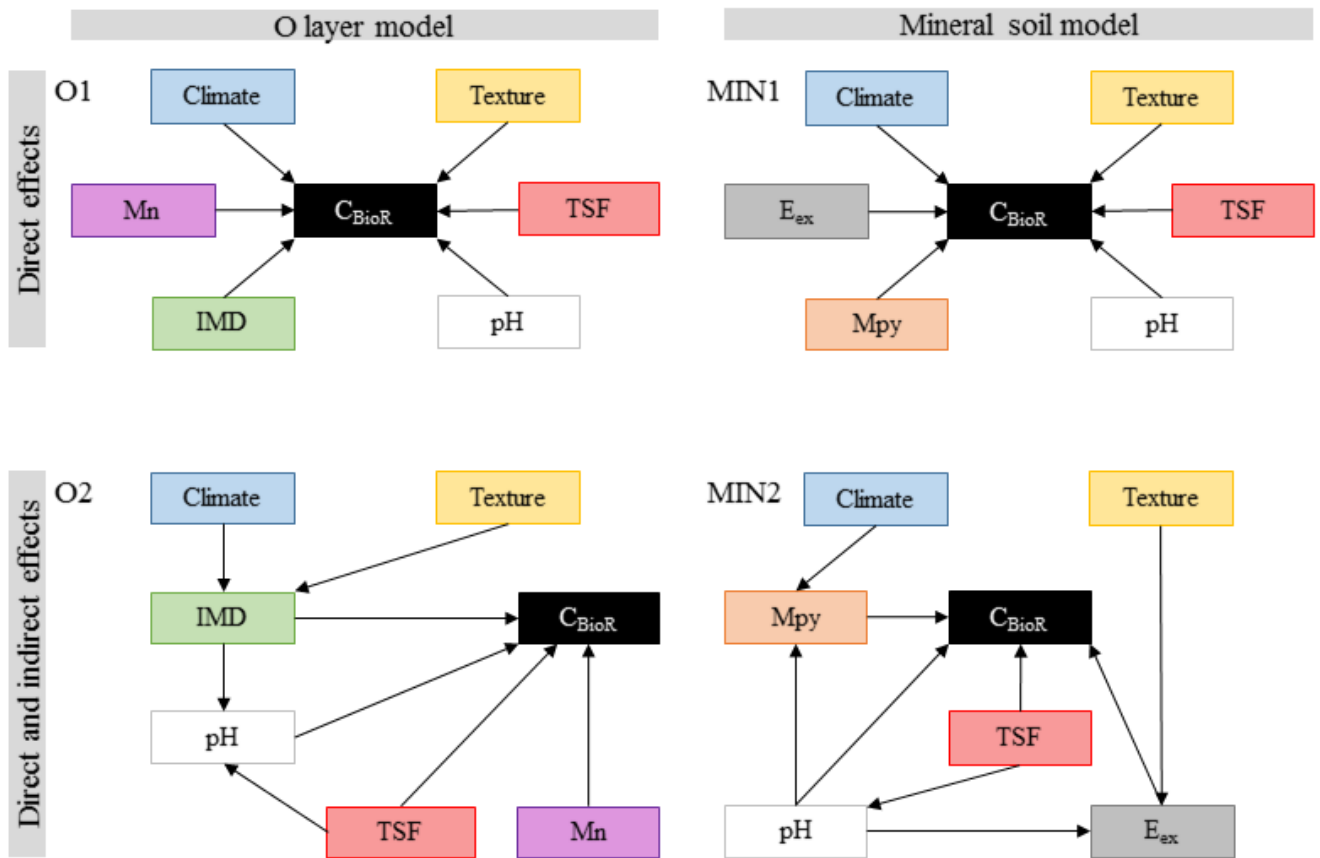
785 Figure 2: Path models for each of the multivariate causal hypotheses. Arrows indicate direct causal relationships. Climate : climate variable; Texture : texture variable; TFS : time since fire; pH : pH of the O layer (O1 and O2) or of the top 35 cm of mineral soil (MIN1 and MIN2); IMD : index of moss dominance; Mn : exchangeable manganese of the O layer; Mpy : pyrophosphate extractable metals; E ex : exchangeable element (Al or Mn) of the mineral soil.
