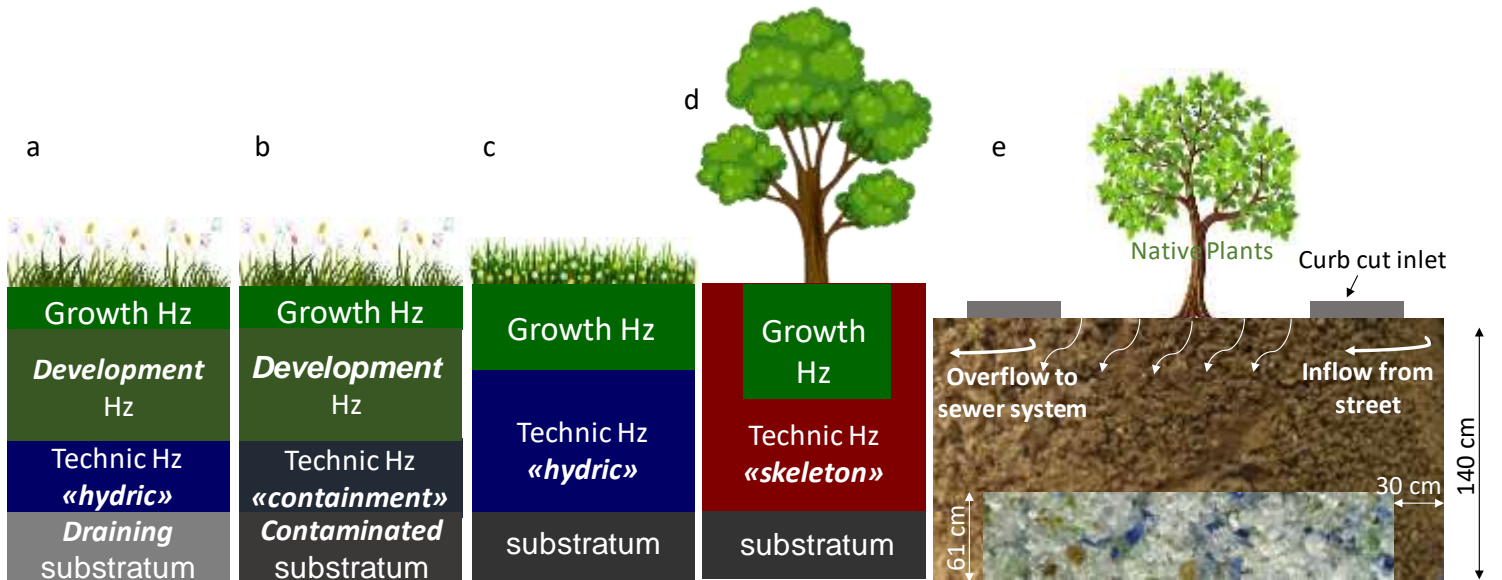
Figure 3: Examples of the organization of horizons in constructed Technosols noted in literature for: a & b) extensive grassland (Biotechnosol project), c) parks and square lawns, d) tree-lined streets (c and d from SITERRE project), e) stormwater management system (DEPNY, 2010).
