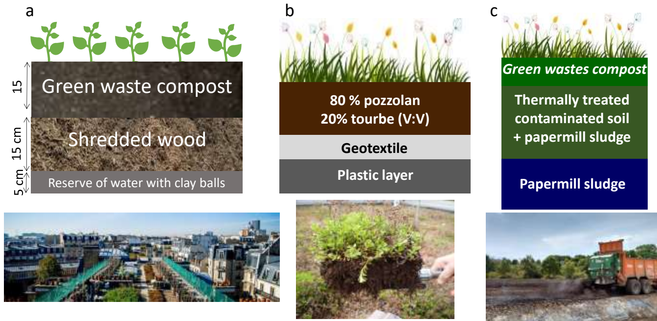
Figure 4: Examples of the organization of horizons in constructed Technosols noted in literature for: a) green roof (Gerard et al., 2018), b) green roof (Bouzouidja et al, 2018), c) abandoned land (Séré et al., 2010).
