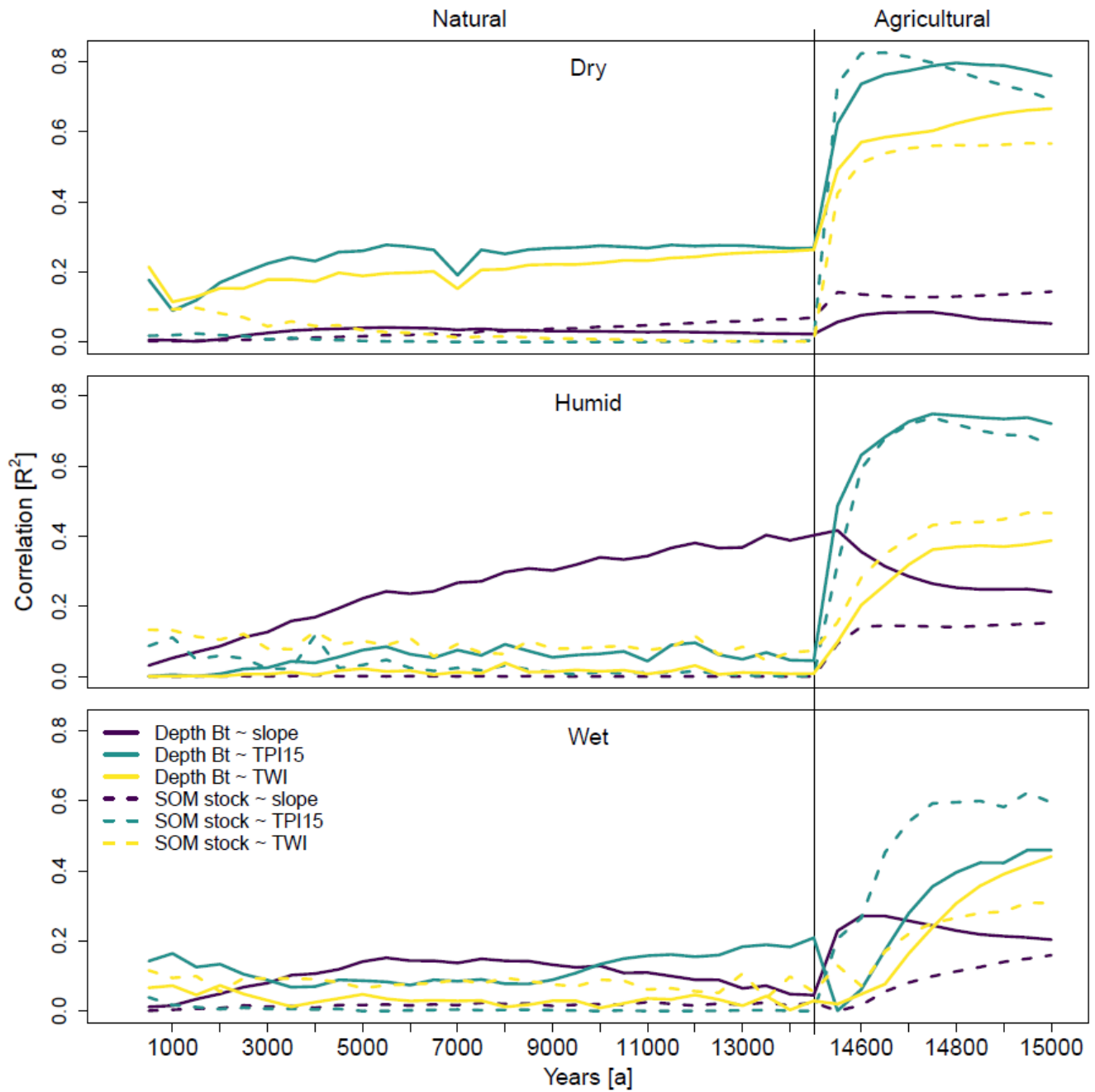
1040 Figure 7: Correlations ( R^2 ) between selected soil properties (line types) and topographic properties (colors) through time (left to right), for the different rainfall scenarios (top to bottom). In the natural system, the correlations are presented every 500 years, while in the agricultural system, the correlations are presented every 50 years. Note that for the latter phase the x-axis is stretched.
