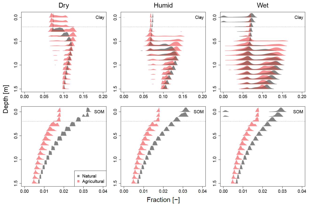
1020 Figure 4: Probability Density Functions (PDFs) showing the multi-modal distributions of soil properties throughout the catchment per 10 cm depth increment. We only show probabilities larger than 5% for clarity. The presented soil properties are clay fraction (top) and SOM fraction (bottom), for the different rainfall scenarios (columns). Grey colors represent the natural soils, while red colors represent agricultural soils. The horizontal dotted line indicates the ploughing depth used for simulations (20 cm).
