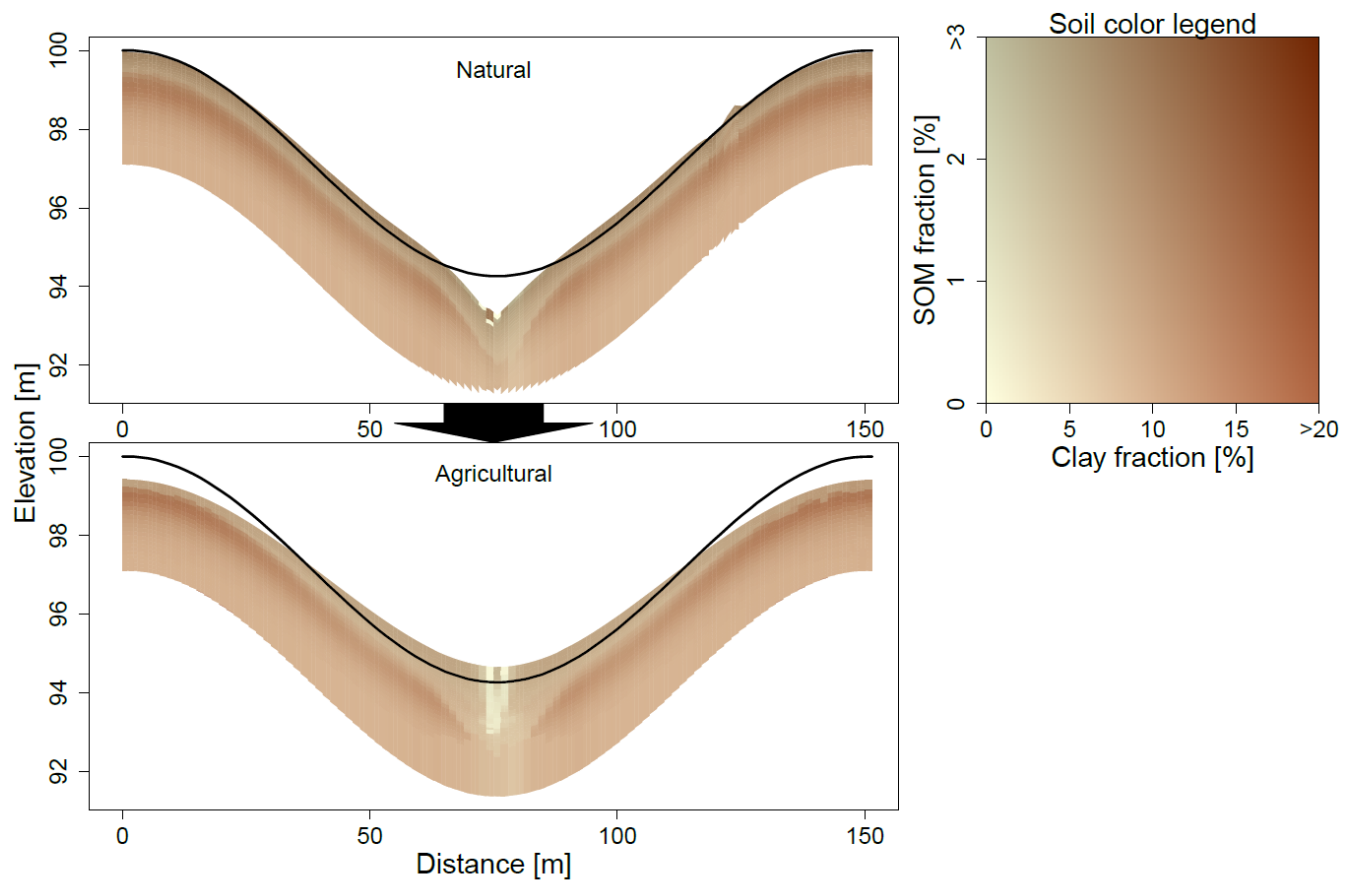
1010 Figure 2: Transect through the catchment at the end of the natural phase and the end of the agricultural phase for the humid scenario ( P = 600 mm). The black line indicates initial topography. See Figure 1 for location of the transect.
