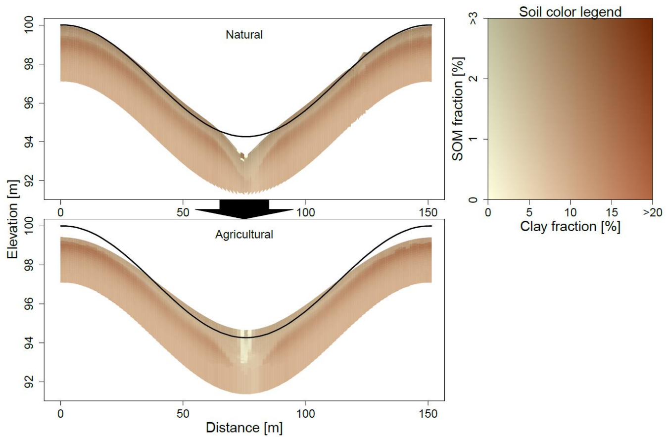
975 Figure 2: Transect through the catchment at the end of the natural phase and the end of the agricultural phase for the humid scenario ( P = 600 mm). The black line indicates initial topography. See Figure 1 for location of the transect.
