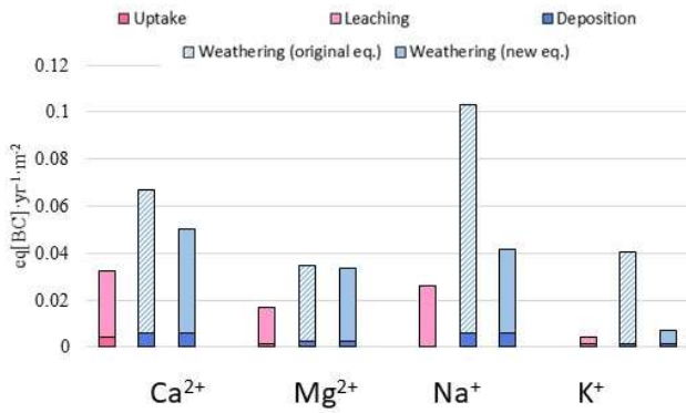
Figure 68. Sinks and source terms of the base cation mass balance for a hillslope. The first bar (pink colours) represents sink terms (net tree uptake and runoff), the second bar represent the source terms with weathering calculated from the original PROFILE equations (model 1), and the third bar represent the source terms with weathering calculated from the new PROFILE equations (model 3).
