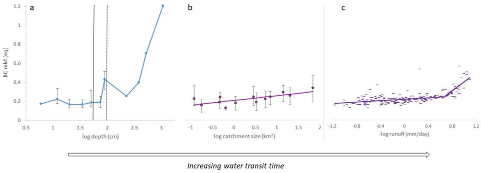
Figure 31. Base cation concentrations (mM-eq) plotted against different proxies for water transit time. a) Soil water concentrations in the S22 soil profile (22 m from stream C2), sampled from 6 cm to 10.7 m depth below surface. Uncertainty bars represent the minimum and maximum concentration observed under eight years of sampling (N = 45-69). Vertical lines represent the approximate highest and lowest groundwater surface depth. b) Stream water concentrations in samples from 2016 (N = 19-25) from the Krycklan basin, plotted against subcatchment size (range from 0.12 to 67 km 2 ). Uncertainty bars represent the minimum and maximum concentration observed during sampling. c) Stream water concentrations in samples 2003-2012 from stream C2 (0.12 km 2 ), plotted against the negative logarithm of runoff. Note that stream C2 displayed in c) is the same as the smallest stream in b), but for two different sampling periods.
