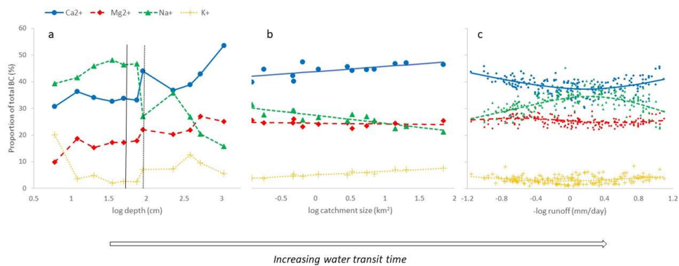
Figure 42. Base cation ratios (%) plotted against different proxies for water transit time. a) Ratios in soil water samples from a soil profile 22 m from stream C2, sampled from 6 cm to 10.7 m depth below surface. b) Ratios in stream water samples from 2016 (N = 19-25) from the Krycklan basin, plotted against subcatchment size (range from 0.12 to 67 km 2 ). c) Ratios in stream water samples 2003-2012 from stream C2 (0.12 km 2 ), plotted against the negative logarithm of runoff.
