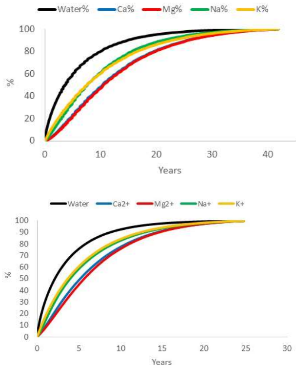
Figure 97. Cumulative water transit time distribution (black) of the study hillslope, and the distribution of "age" of the water carrying each of the base cations according to model 3.
