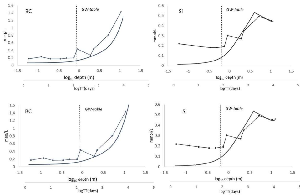
Figure 64. Modelled BC (left) and Si (right) concentrations from model 2, plotted against \log_{10} of WTT (smooth lines). Overlain are the observed BC and Si-concentrations from the soil profile, plotted against \log_{10} of soil depth (straight lines with markers). Note that the scales are not directly comparable, instead the figures are intended to illustrate trends and ranges of solute concentrations.
