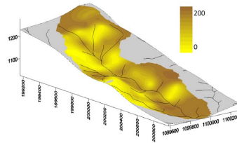
Figure 4. Map of the thickness of the andic material layer (in cm) in the AQUIARES watershed. The vertical scale indicates elevation (in meters) above sea level. Numbers on x and y axes are UTM coordinates.
