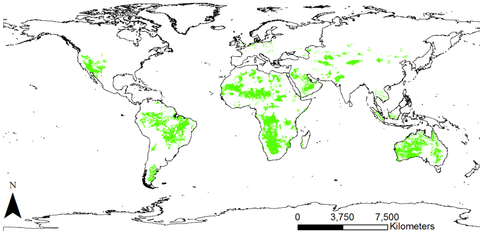
5 Figure 3: Overview of locations suitable for making soil peels in the world (sand content > 70%, clay content < 15%, organic matter < 8%, and temporal mean groundwater depth < 1.5 m). This global map was made using soil information obtained from ISRIC (Batjes, 2012; ISRIC, 2018a) and groundwater depth information provided by Fan et al. (2013).
