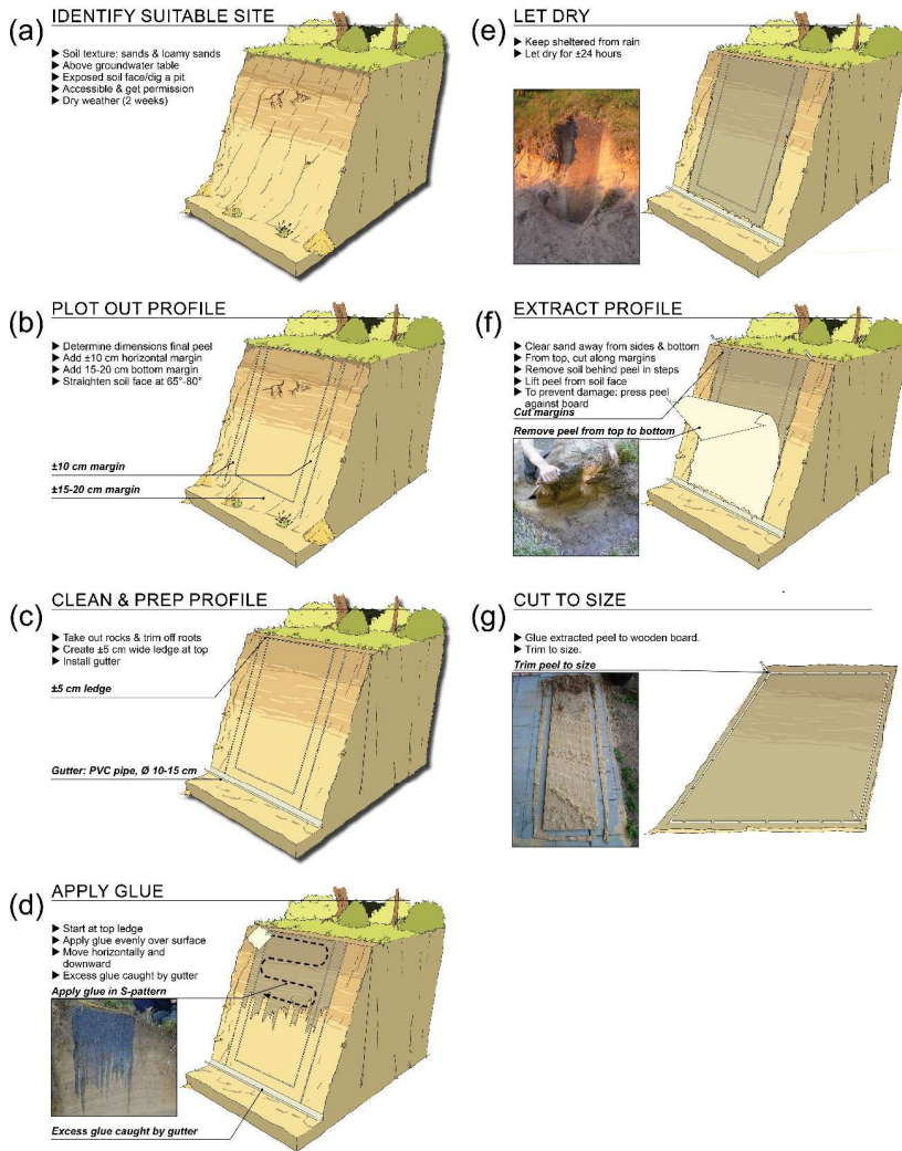
Figure 2: Main steps of making a soil peel
