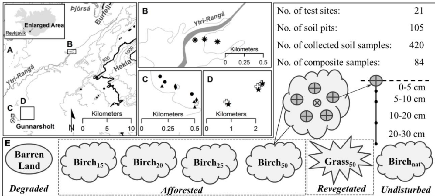
5 Figure 1: The topological map (equidistance = 100 m) showing the study area between the Ytri-Rangá River, Mount Burfell, Mount Hekla and Gunnarsholt (crossed cycle) in the south of Iceland (A). The locations of the naturally growing birch woodland (B; asterisks) and the afforested (C; B15: circles, B20: triangles; B25: pentagons; B50: diamonds) and degraded (crosses) as well the revegetated (stars) test sites (D) are shown in more detail. The sampling scheme illustrates the age and vegetation characteristics of the different study sites and the applied soil sampling setup (E).
