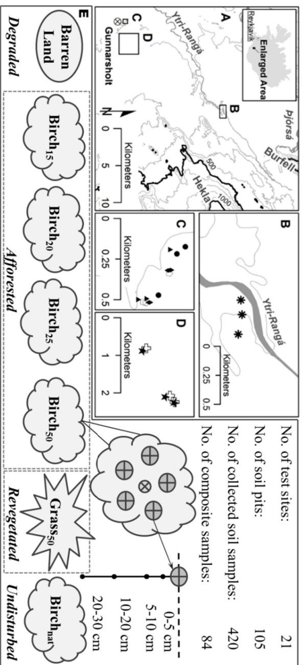
Figure 1: The topological map (equidistance = 100 m) showing the study area between the Ytri-Rangá River, Mount Burfell, Mount Hekla and Gunnarsholt (crossed cycle) in the south of Iceland (A). The locations of the naturally growing birch woodland (B; asterisks) and the afforested (C; B15: circles, B20: triangles; B25: pentagons; B50: diamonds) and degraded (crosses) as well as the revegetated (stars) test sites (D) are shown in more detail. The sampling scheme illustrates the age and vegetation characteristics of the different study sites and the applied soil sampling setup (E).
