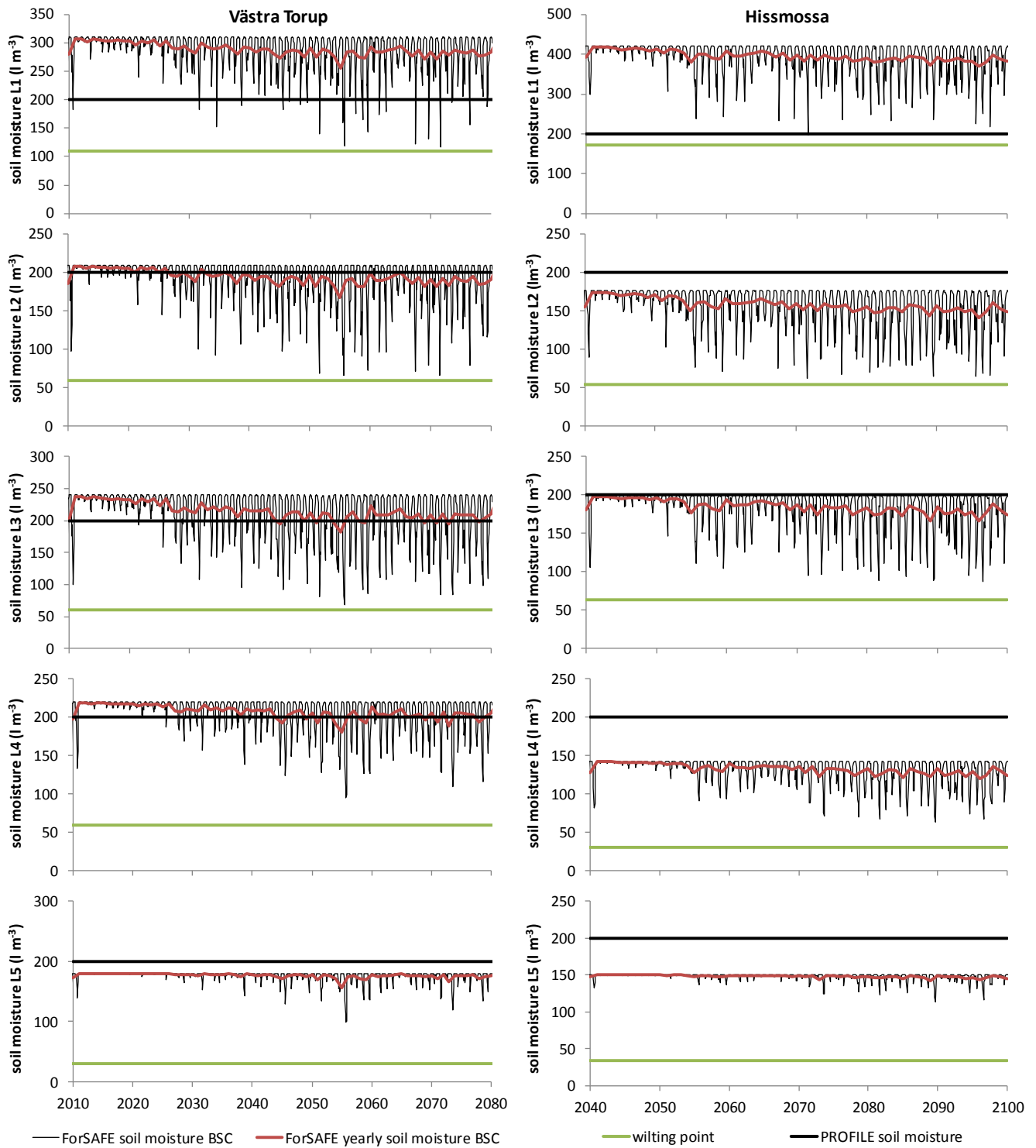
Figure 2. Soil moisture in all soil layers, BSC scenario, forest rotation 2010-2080 in Västra Torup and 2040-2100 in Hissmossa, compared to wilting point and PROFILE input soil moisture.
