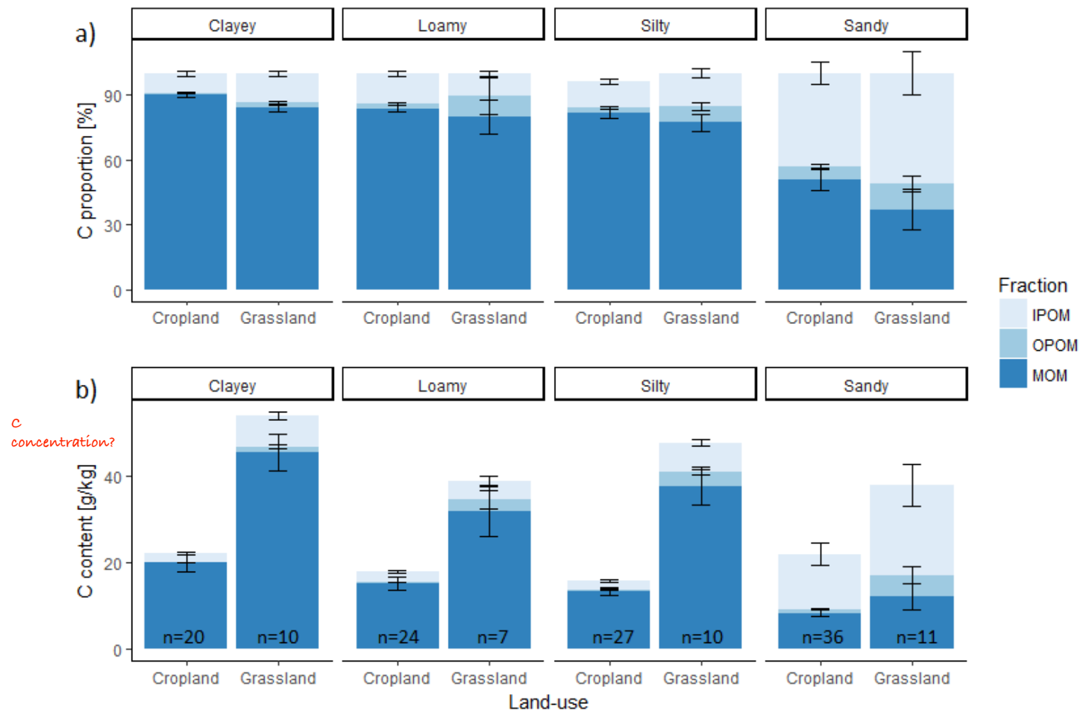
Fig. 2: a) Proportion (%) and b) absolute content ( \text{g kg}^{-1} ) of soil organic carbon (SOC) in the intra-aggregate particulate organic matter (iPOM), occluded particulate organic matter (oPOM) and mineral-associated organic matter (MOM) fraction in different soil texture classes for the 145 calibration sites that were fractionated. Error bars denote the standard error of the mean.
