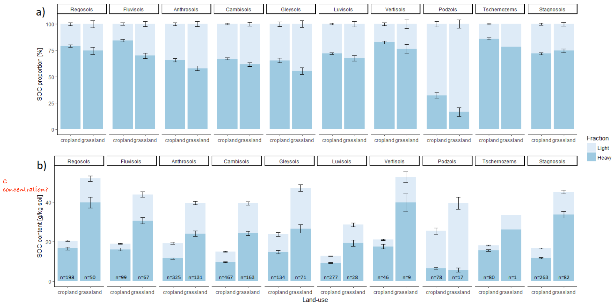
Fig. 6: a) Proportion (%) and b) absolute content ( \text{g kg}^{-1} ) of soil organic carbon (SOC) in the light and heavy fractions in different soil types in the 'normal' soils (non-black sands) dataset. Error bars denote standard error of the mean.
