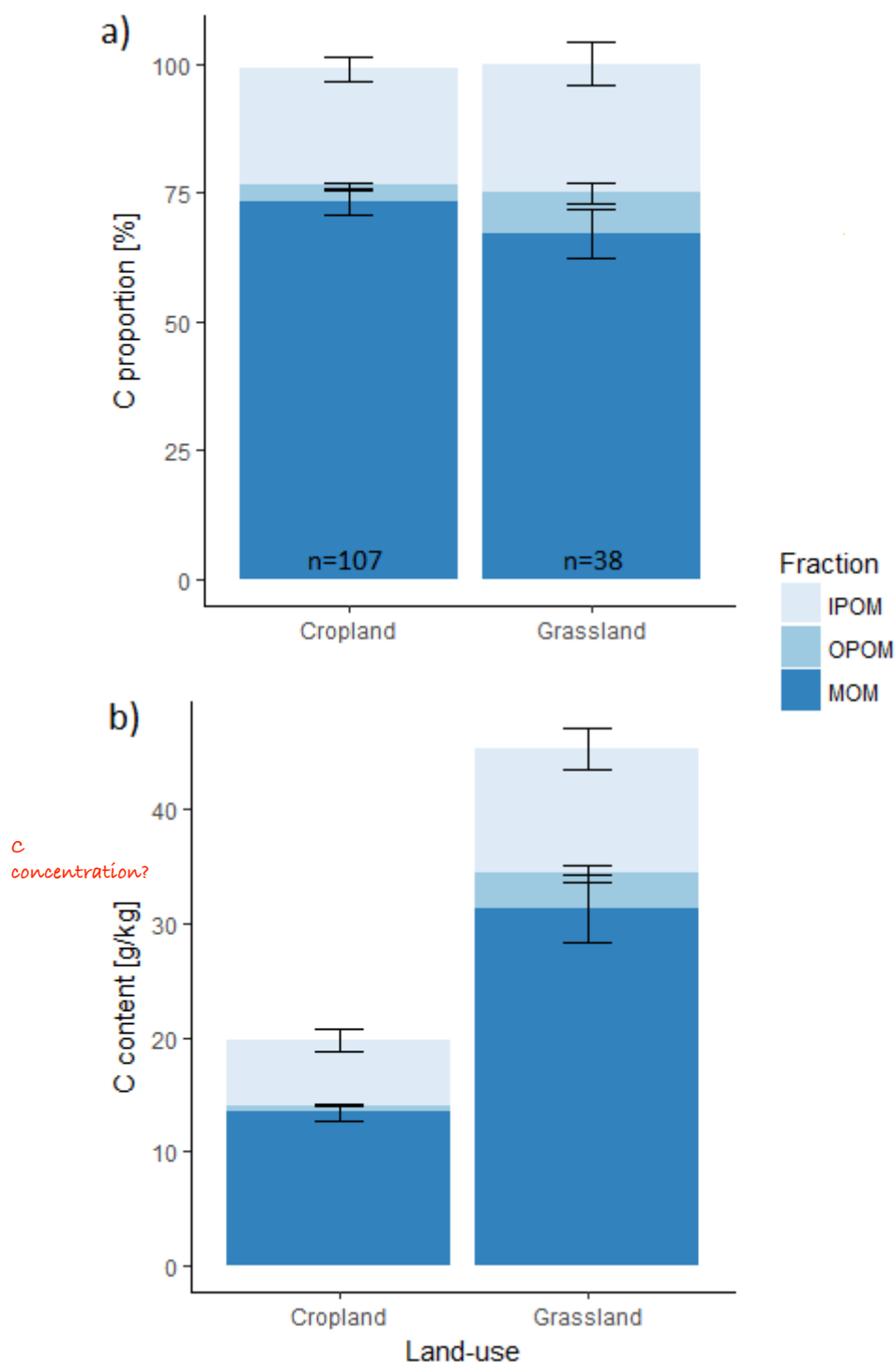
Fig. 1: a) Proportion (%) and b) absolute content ( \text{g kg}^{-1} ) of soil organic carbon (SOC) in the intra-aggregate particulate organic matter (iPOM), occluded particulate organic matter (oPOM) and mineral-associated organic matter (MOM) fraction in soils under cropland and grassland for the 145 calibration sites that were fractionated. Error bars denote standard error of the mean.
