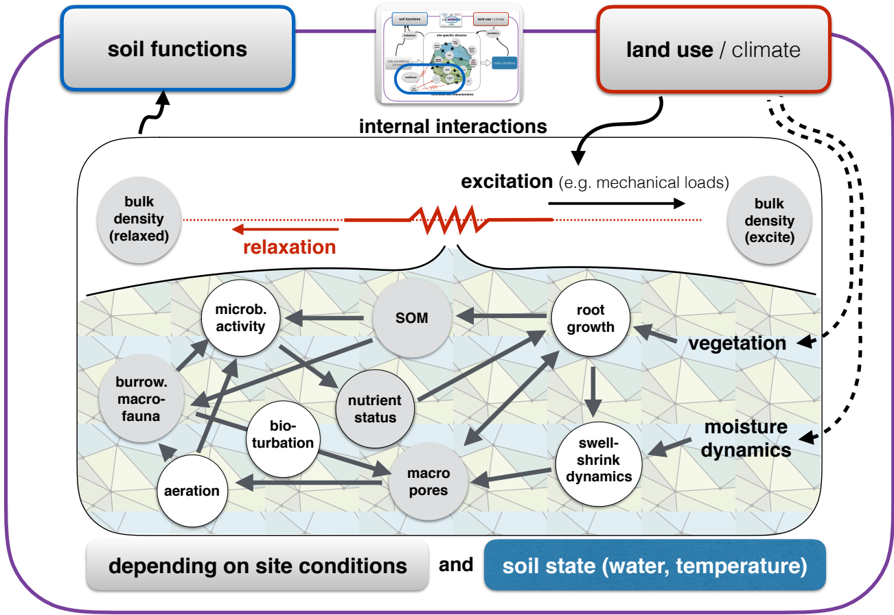
Figure 4. Zoom into Fig. 3: The excitation (i.e. disturbance) of the soil system by compaction due to mechanical loads is relaxed by interacting processes at the smaller scale. The functional characteristics considered for this case are indicated by grey circles while the connecting processes are in white.
