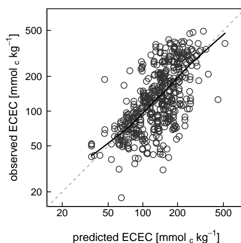
Figure 3. Scatter plot of measured against predicted ECEC in 0–20 cm mineral soil depth, computed with geoGAM (Sect. 4.1.1) for the sites of the validation set (solid line: loess scatter plot smoother, n: number of measurements).
