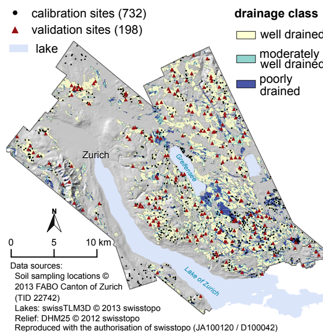
Figure 7. geoGAM predictions of drainage classes for the agricultural land in the Greifensee study region (computed on a 20 m-grid with final geoGAM with covariates according to Table 2, smoothed for better display with focal mean with radius of 3 pixels = 60 m). Black dots are locations used for geoGAM calibration, locations with red triangles were used for model validation.
