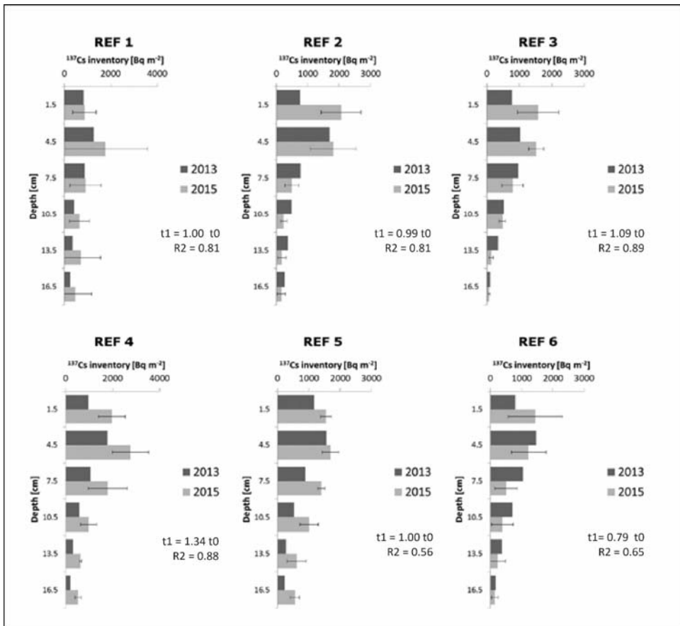
295 Figure 7: The ^{137}\text{Cs} depth profiles of the six investigated reference sites in the Urseren Valley for the two different sampling campaigns. The errors bars indicate the standard deviations of the inventories among the replicates collected at each reference site in 2015. Further, the regression equation between the depth profile at t_0 and t_1 is displayed together with the R^2 .
