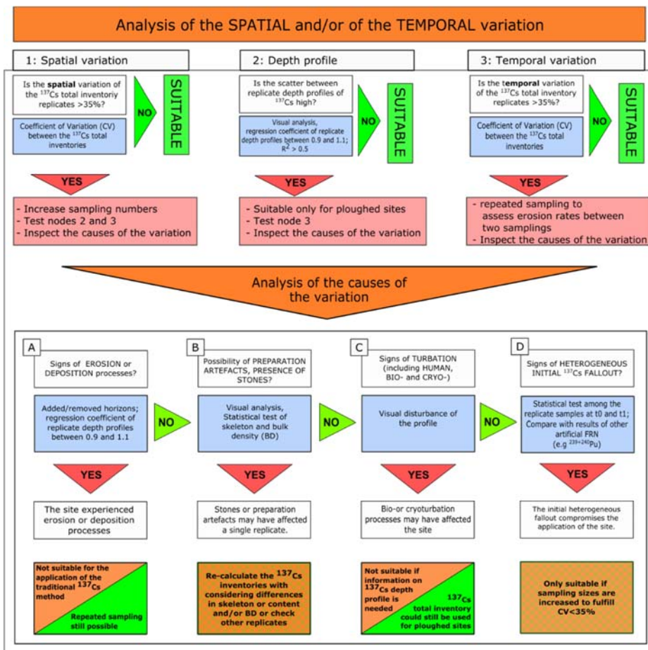
Figure 2: The CheSS decision tree to evaluate the suitability of a reference site for using 137 Cs as a soil erosion tracer.
