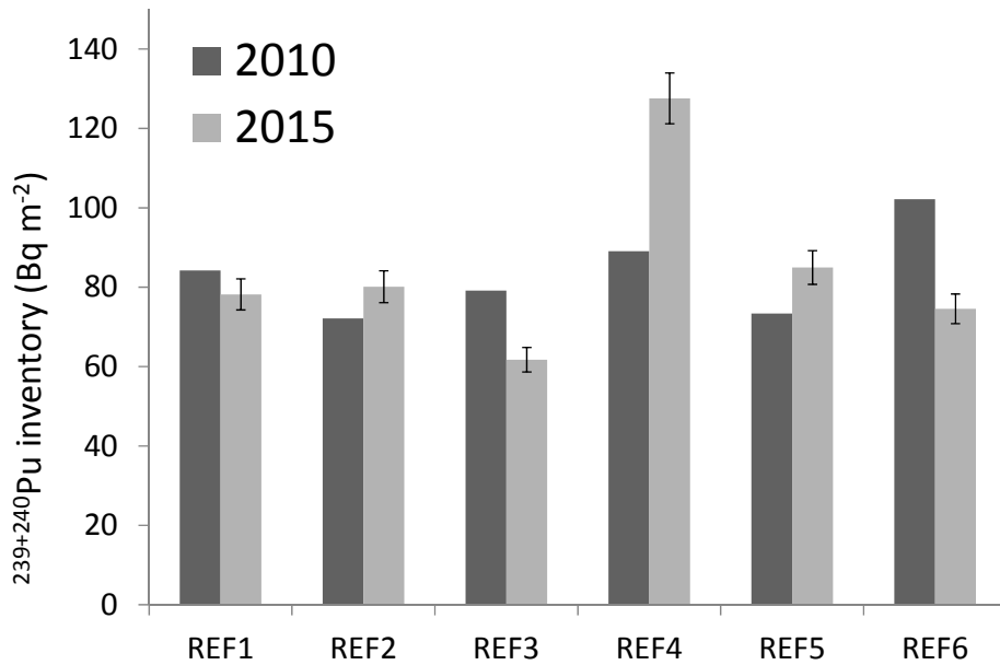
Figure 8: Temporal variation between the total 239+240 Pu inventories measured at the reference sites in the Urseren Valley, where Time 0 = 2010 and Time 1 = 2015. The errors bars indicate the standard deviations of the inventories among the replicates collected at each reference site in 2015.
