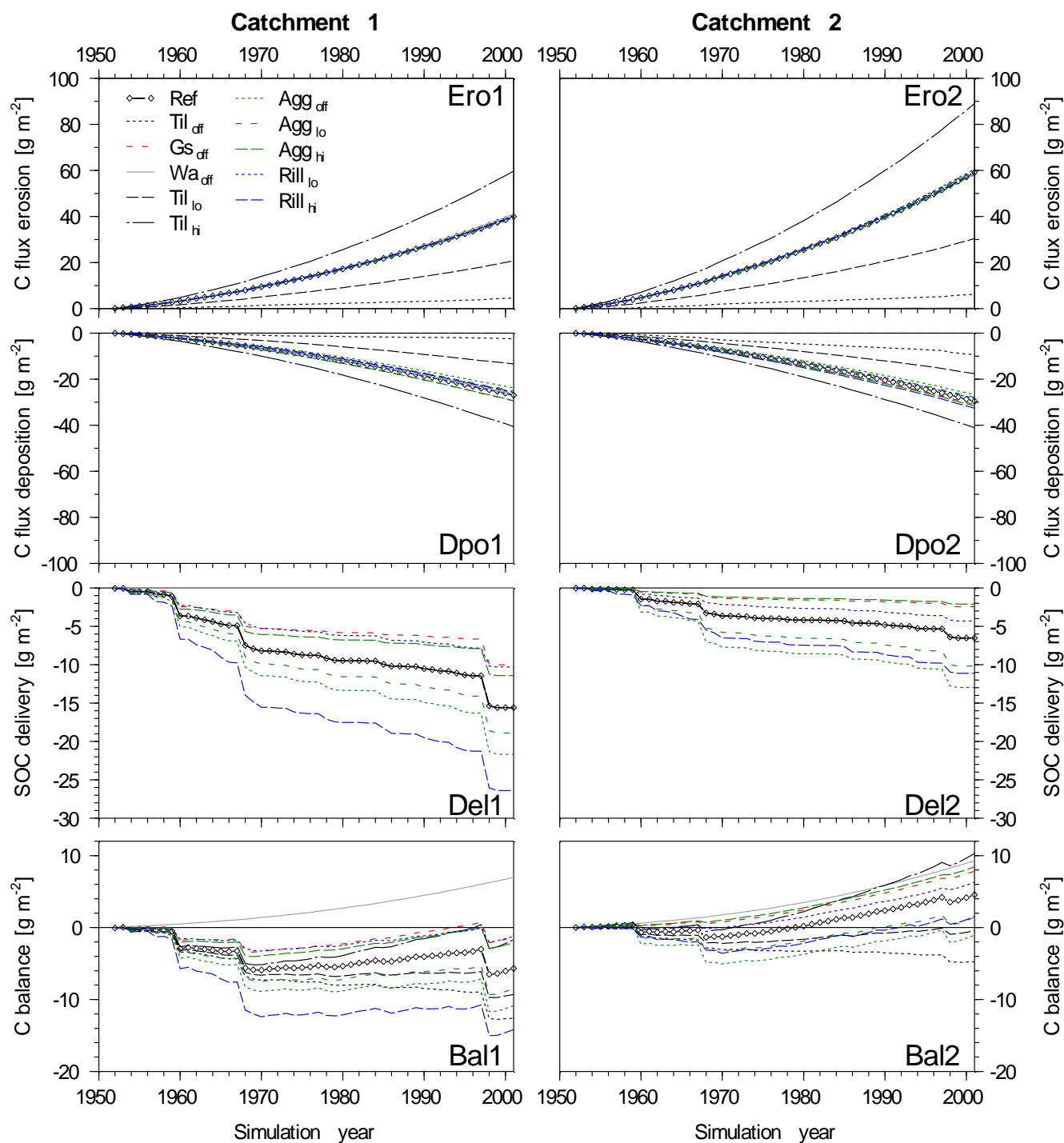
Figure 5: Simulated cumulative vertical C fluxes for erosional (Ero1, Ero2) and depositional (Dpo1, Dpo2) sites; lateral C delivery (Del1, Del2) and overall catchment C balance (Bal1, Bal2) for catchment C1 and C2. For details regarding the model runs and corresponding abbreviations see Table 2.
