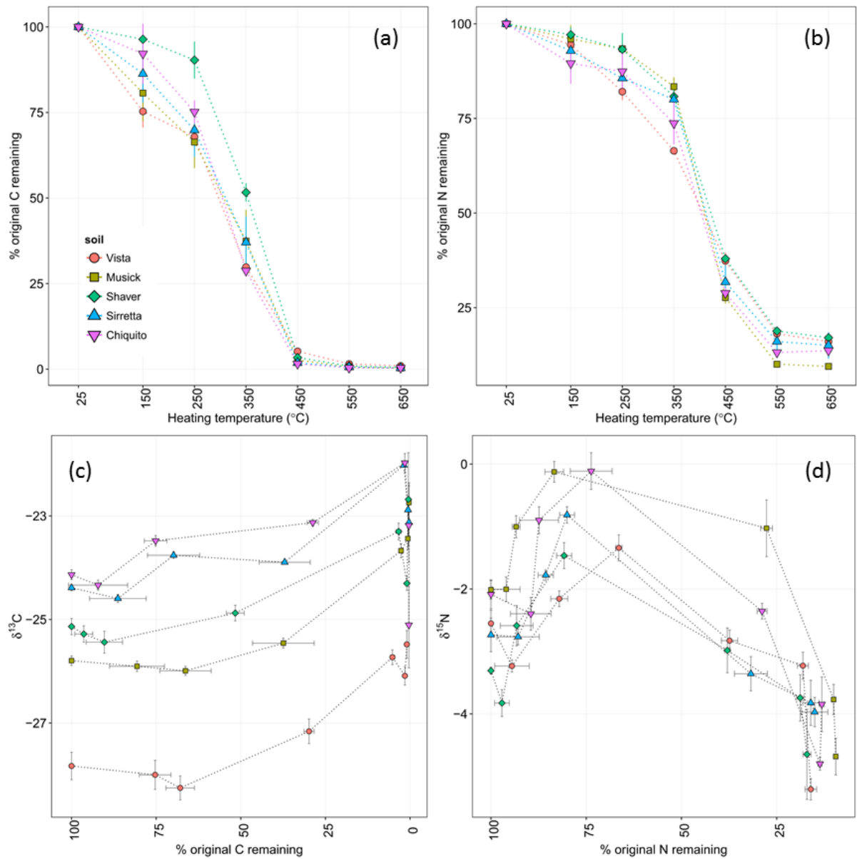
Figure 6: (a) Percentage of C and (b) N loss with heating; and (c) change in \delta^{13}\text{C} and (d) \delta^{15}\text{N} versus percent of total C and N lost from soils (error bars represent standard error where n=3).
