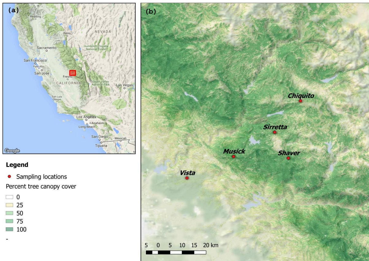
Figure 1: (a) Location of the sampling site on the western slopes of the Sierra Nevada, California, and (b) map of the five sampling locations and percent tree canopy cover (U.S. Geological Survey, 2014).
