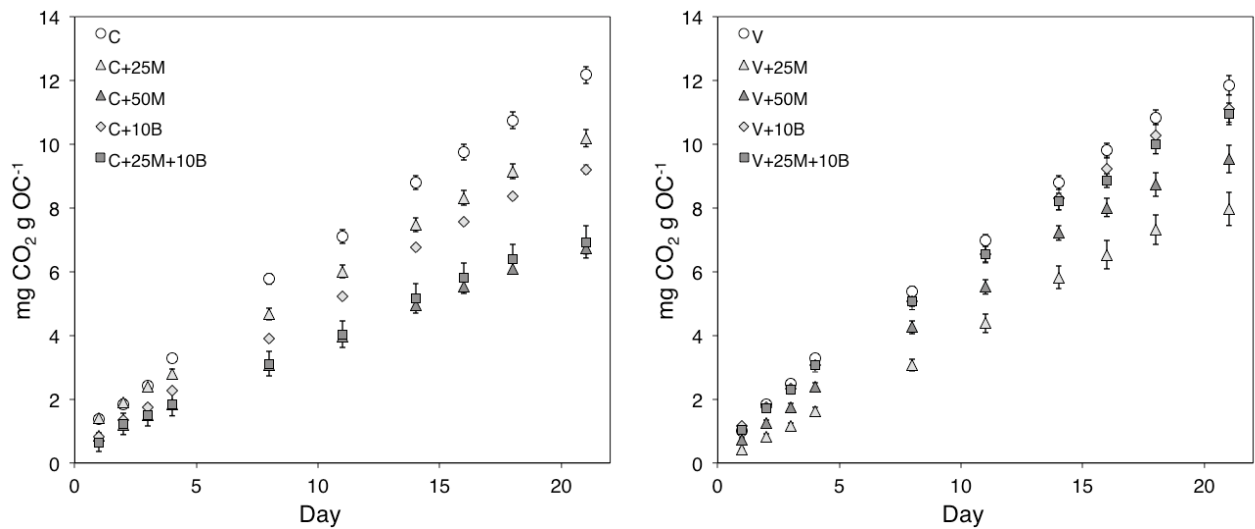
605 Figure 2. A) Cumulative CO 2 emissions during composting without worms of pre-composted material alone (C), with 25% of clay (C+25M), with 50% of clay (C+50M), with 10% of biochar (C+10B) or with 25% of clay and 10% of biochar (C+25M+10B). B) Cumulative CO 2 emissions during composting with worms of pre-composted material alone (V), with 25% of clay (V+25M), with 50% of clay (V+50M), with 10% of biochar (V+10B) or with 25% of clay and 10% of biochar 610 (V+25M+10B). Bars represent twice the standard deviation of the mean (n=4).
