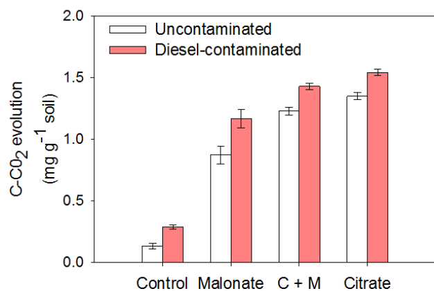
10 Figure 1: Cumulative CO 2 evolved over the 18-day incubation in diesel-contaminated and uncontaminated soils which received water (control) or 5 μmol g -1 soil of citrate, malonate, or citrate + malonate every 48 hours. Values are means ± SE (n=4). There was an effect of carboxylate addition ( P<0.001 ) and diesel-contamination ( P<0.001 ), but no significant interaction.
