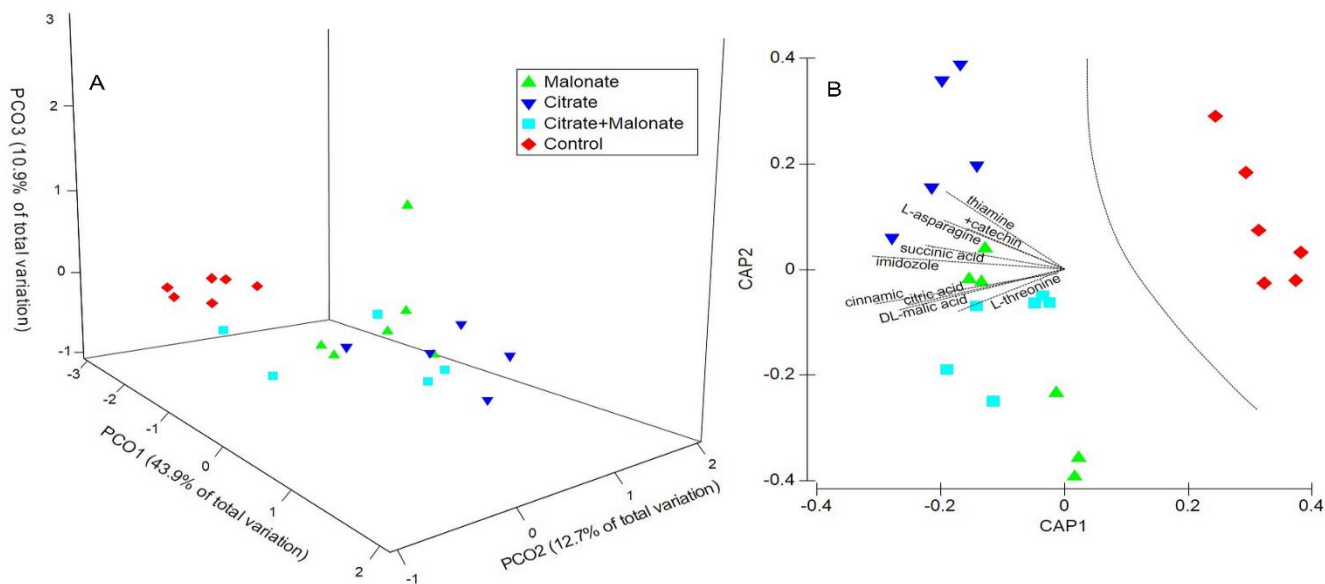
5 Figure 2: (a) Principal co-ordinate analysis ordination (PCO) and (b) canonical analysis of principal co-ordinates (CAP) of CLPP on soil after 18 days of incubation for diesel-contaminated and uncontaminated soils which received water (control) or 5 \mu\text{mol g}^{-1} soil of citrate, malonate, or citrate + malonate every 48 hours. As there was no effect of diesel-contamination there is no distinction made between the three replicates of each carboxylate treatment from diesel-contaminated soil and the three replicates from uncontaminated soil. The curve in Fig. 2 (b) represents a significant difference ( P_{\text{Perm}}=0.004 based on PERMANOVA) between treatments receiving carboxylates and the water control.
