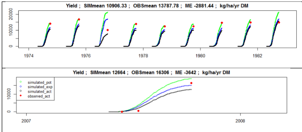
5 Figure 6. Results of simulated and observed yields of silage maize: Cranendonck 16 (upper figure) and Dijkgraaf (lower figure). The green lines correspond with the simulated potential yield; blue with the simulated exploitable yield; black with the simulated actual yield; red dots indicate the observed dry matter yield. SIMmean, OBSmean and ME are annual mean values for simulated actual yield, observed yield and the difference (maximum error ME).
