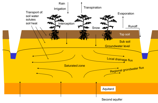
Figure 1. Transport processes and modelling domain of SWAP.
