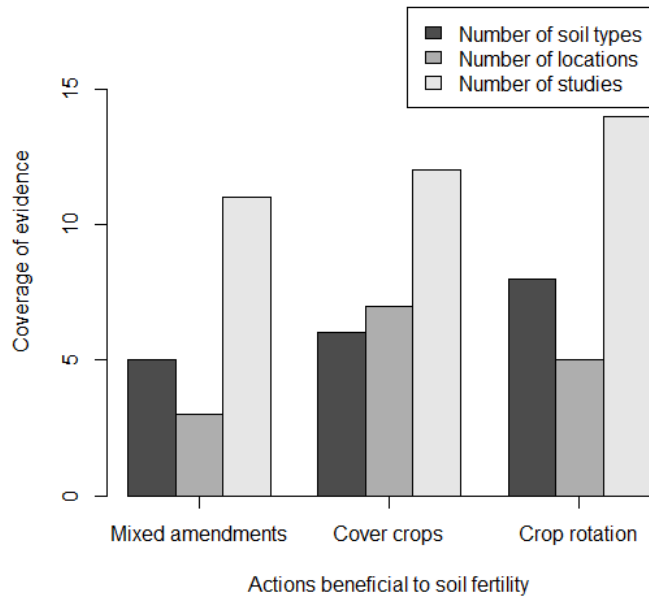
Figure 1. Coverage of soil type, geographical location and number of studies for the three actions/practices identified as beneficial to soil fertility. Mixed amendments = amend with integrated nutrient management (a mix of organic and inorganic amendments); cover crops = grow cover crops when field is empty ; crop rotation = use crop rotation.
