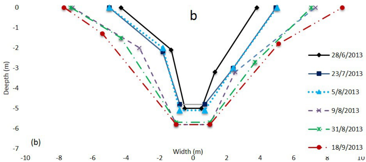
Fig. 3. (a) Cross section segmentation methodology to determine the cross-sectional area of the gullies. (b) Measured profiles of a cross-section located on gully G6 during the 2013 rain phase, showing the lateral and downward expansion of the gully.
