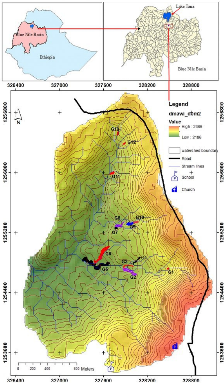
Fig. 2. Location of the Debre Mawi watershed within the Blue Nile River basin, Ethiopia (top figures). The watershed map (bottom) shows the contour lines, elevation, stream lines, and the 13 studied gullies (indicated by the labels beginning with the letter G). Projected Coordinate System:
