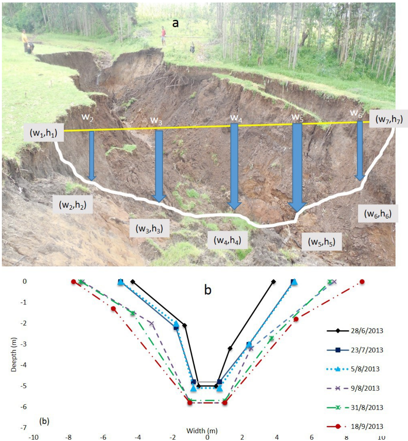
Fig. 3. (a) Cross section segmentation methodology to determine the cross-sectional area of the gullies. (b) Measured profiles of a cross-section located on gully G6 during the 2013 rain phase , showing the lateral and downward expansion of the gully.
