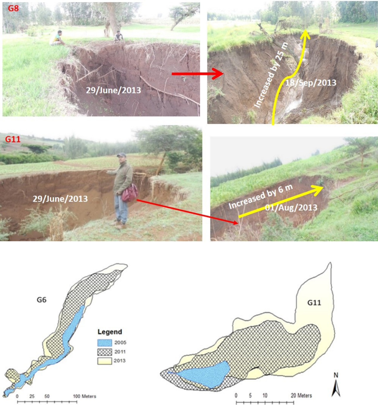
800 Fig. 6. Examples of gully expansion in the Debre Mawi watershed: (Top photo) expansion of gullies G8 and G11 during the 2013 rain phase , the trees which were upstream of the two gullies felled down in to the gullies; (Bottom image) expansion of gullies G6 and G11 between 2005 and 2013.
