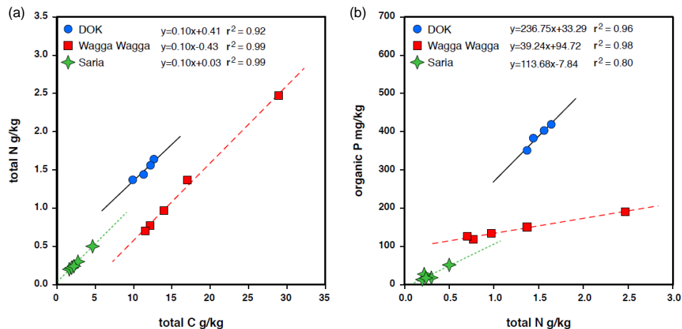
Figure 4. Relationships between soil C and soil N concentrations (a) and between soil N and soil organic P concentrations (b) in the three field experiment. Points in blue represent DOK, points in red represent Wagga Wagga, and points in green represent Sarria. All relations are statistically significant at p < 0.05 .
