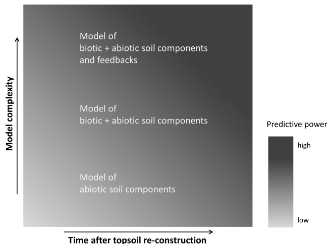
Figure 2. Conceptual scheme of predictive power of soil water models at different levels of complexity. While uncertainty of hydrological variables such as deep drainage or plant available water is lowest for traditional models that only consider abiotic soil components, these models may also have low predictive power due to omission of critical macrofauna – soil structure interactions. Integration of biotic components and feedbacks between macrofauna taxa, and macrofauna and soil development increases model complexity and thereby uncertainty. However, quantification of macrofauna – soil interactions by controlled scientific experiments reduces these uncertainties, thereby increasing the predictive power to a level acceptable to assess the risk of potential failure of post-mining land rehabilitation.
