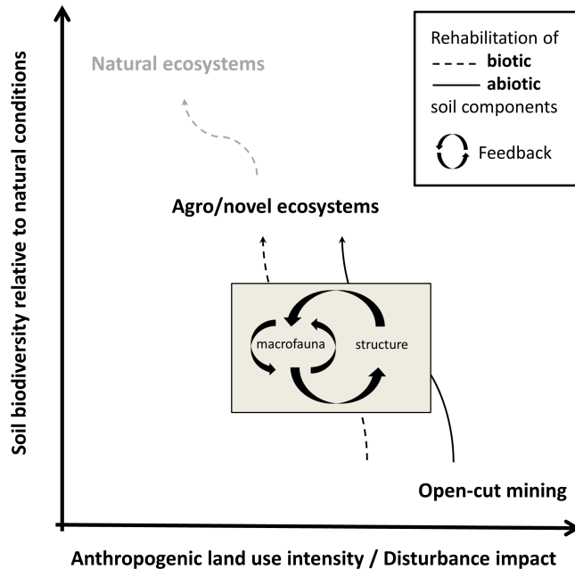
Figure 1. Relation between land use intensity/disturbance impact and soil biodiversity of natural ecosystems, conventional agriculture, and open-cut mining lands (modified after Bottinelli et al., 2015, and Doley and Audet, 2013). While the transition from conventional agriculture to natural ecosystems mainly requires restoration of biotic soil components, the transition of open-cut mining land to novel (Perring et al., 2014), agricultural or native ecosystems (if possible) requires rehabilitation of both biotic and abiotic soil components. Feedbacks between different macrofauna taxa, and macrofauna and soil structure might be critical drivers of the temporal transition of open-cut mining land to novel or agricultural ecosystems.
